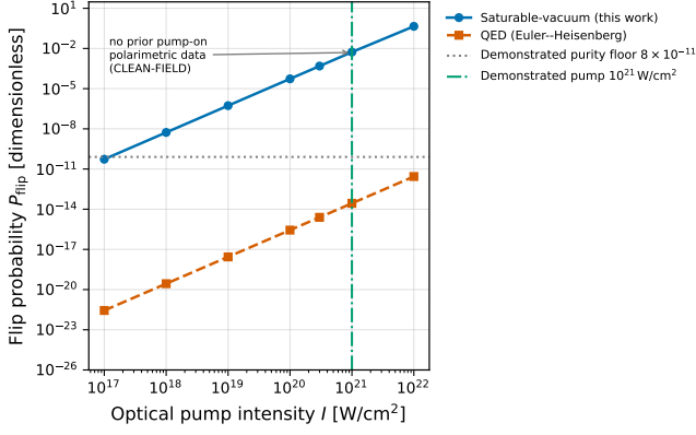
FIG. 1. The exposure plane. Predicted polarization-flip probability P_{\text{flip}} versus optical-pump intensity for the saturable-vacuum model (blue, Eqs. (3) and (8)) and for the QED Euler–Heisenberg co-prediction (orange, Eq. (7)), through the identical single-pass readout chain at probe energy 9835 eV, z = 10 \mu\text{m} . Both scale as intensity squared, so their ratio is field-independent. The dotted line marks the record X-ray-polarimeter purity ( 8 \times 10^{-11} , Ref. [12]; the conservative 2.4 \times 10^{-10} single-measurement floor of Ref. [13] used for the kill criterion lies just above it), and the dash-dot line the demonstrated ReLaX pump ( 10^{21} \text{ W cm}^{-2} ). No prior experiment occupies the pump-on polarimetric exposure region, so the model’s prediction there is unconstrained by existing data.
