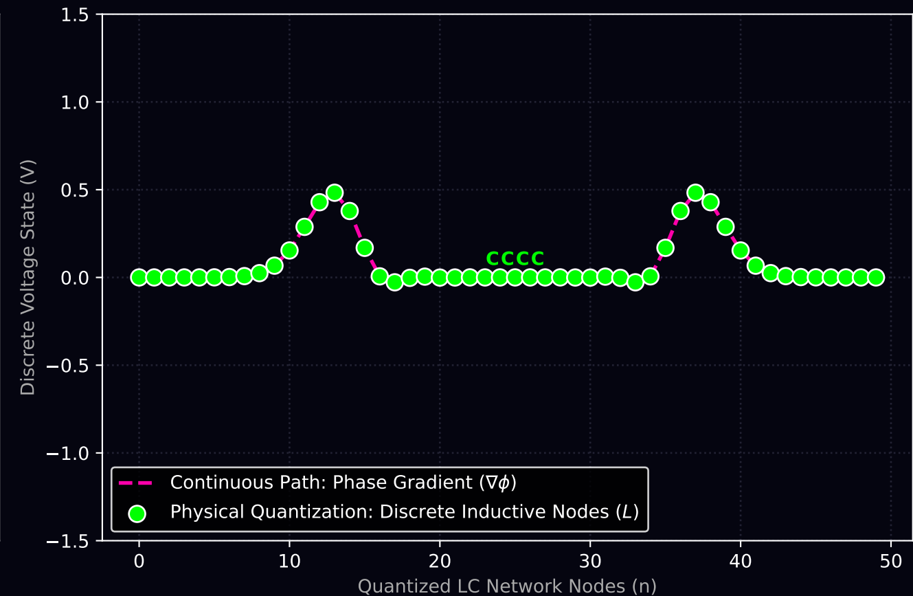
AVE Reality: Discrete LC FDTD Solvers
