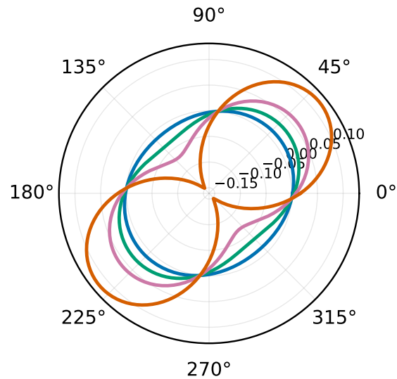
random control (quadratic): \omega/(c|k|) - 1 vs direction
