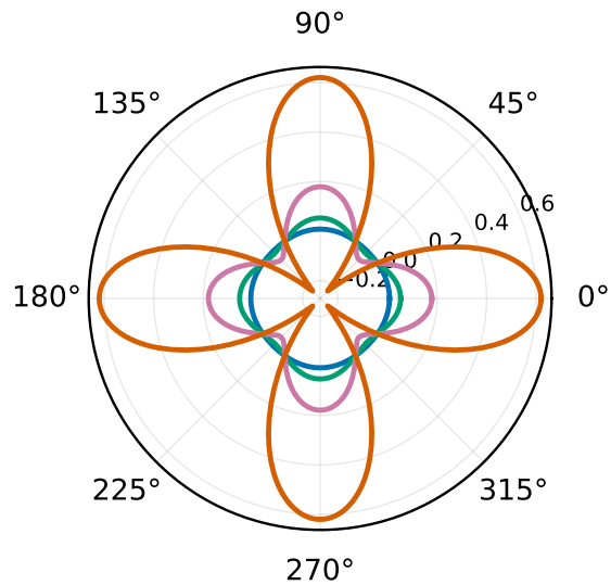
K4 photon (quartic): \omega/(c|k|) - 1 vs direction
