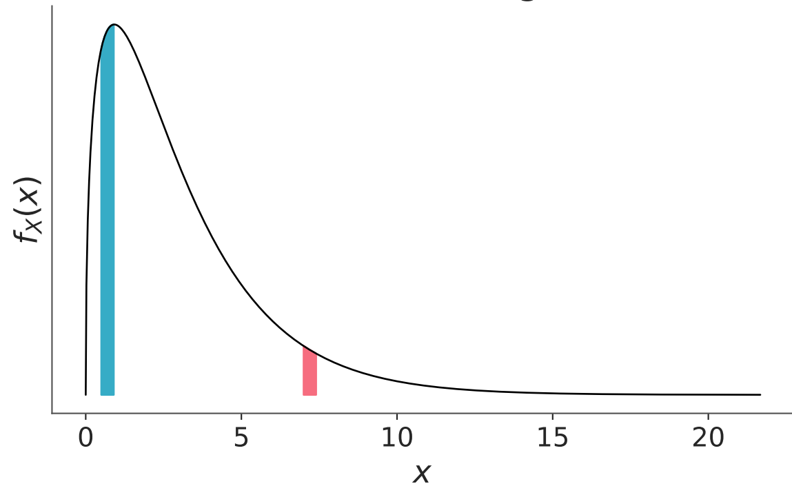
X \sim \text{Gamma}(\mu=3, \sigma=2.5)
