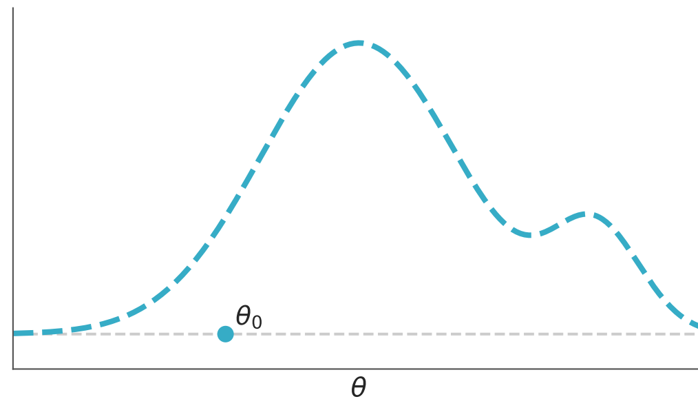
Evaluate the target density
