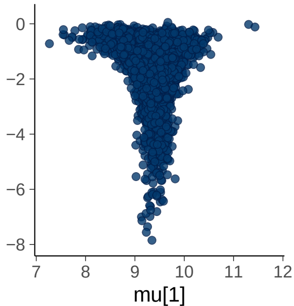
NCP + adapt_delta=0.9
