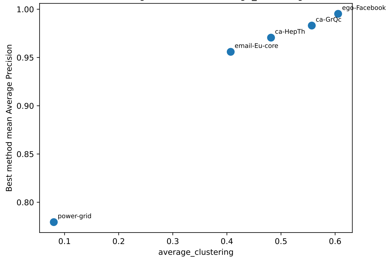
Best Average Precision vs average_clustering
