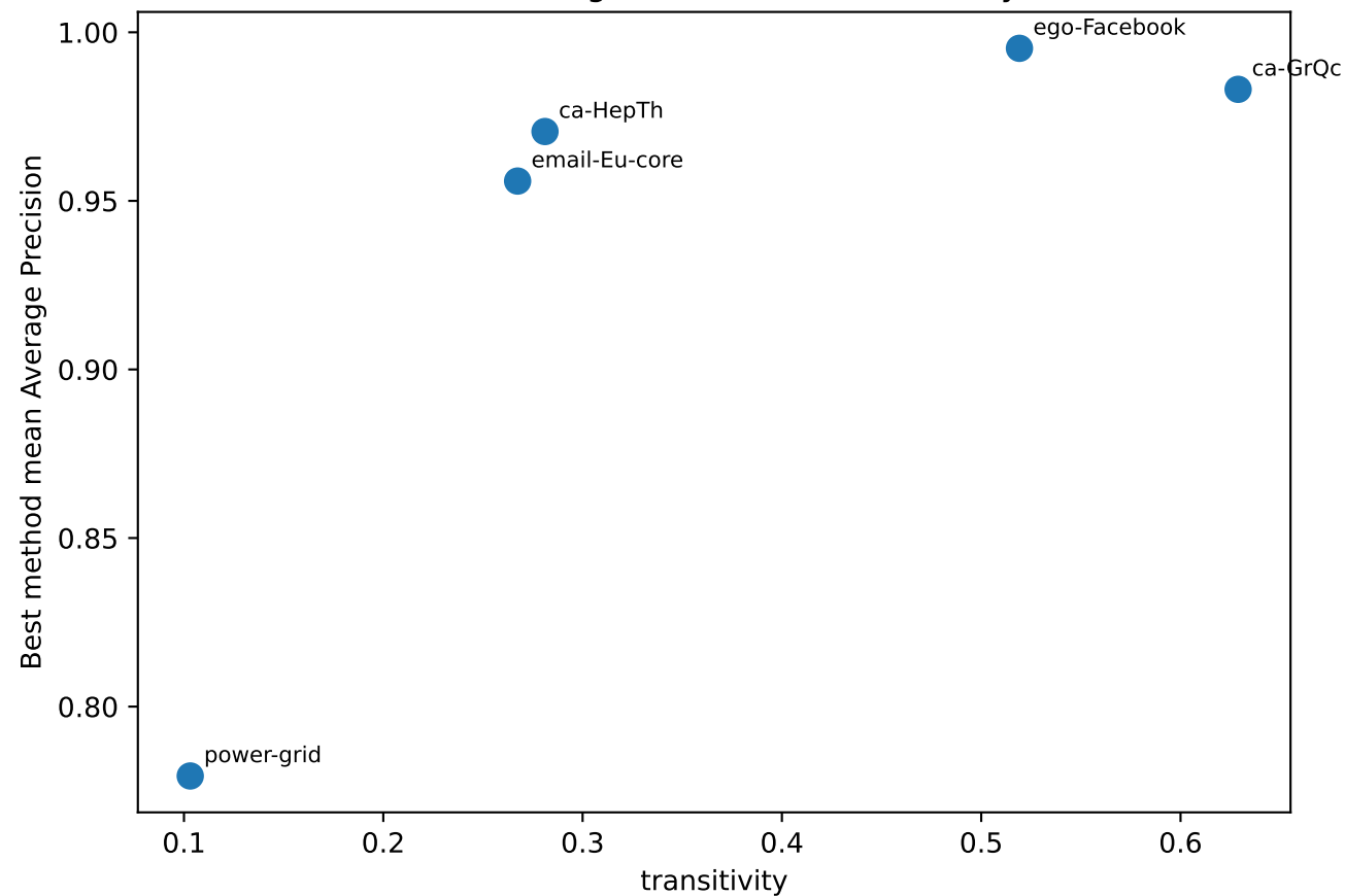
Best Average Precision vs transitivity
