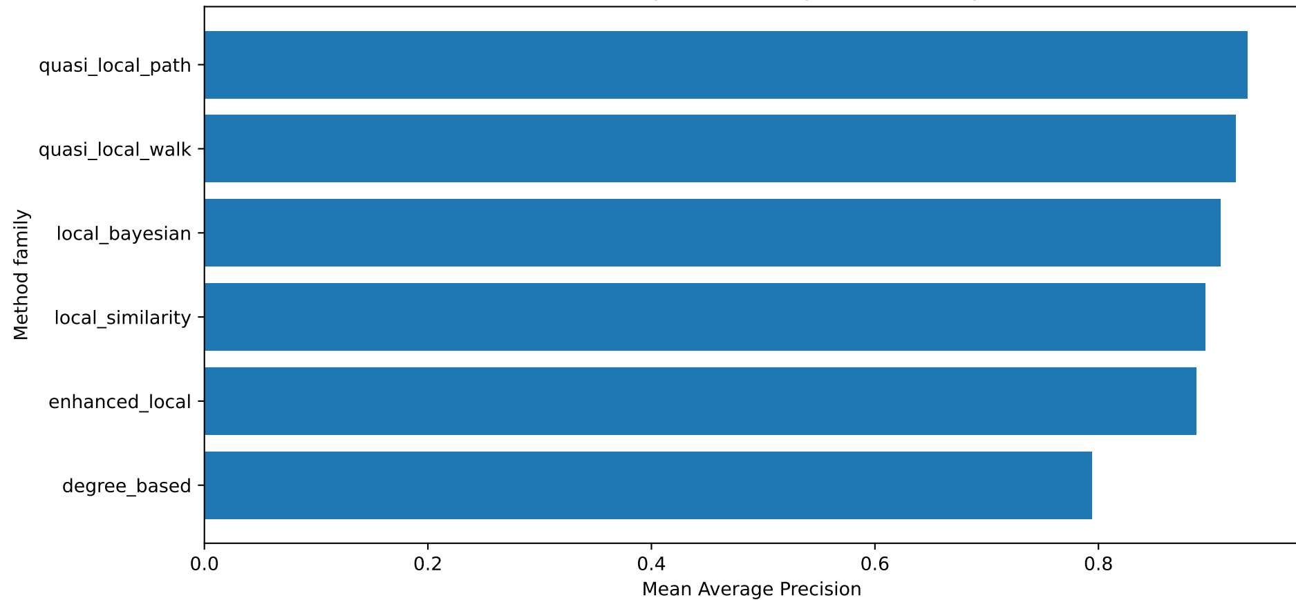
Mean Average Precision by method family
