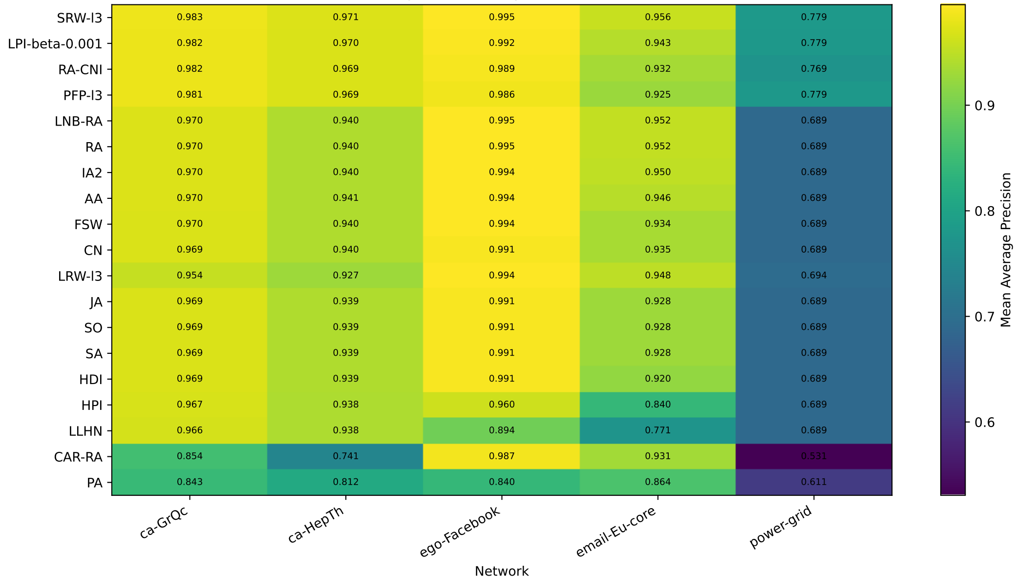
Mean Average Precision by method and network
