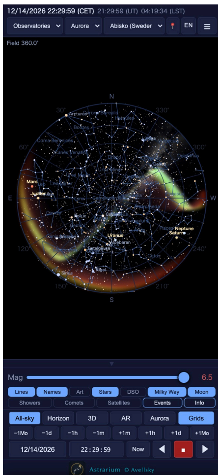
Figure 16. An auroral breakup in progress — ten minutes from onset, the bulge rising poleward and running west
