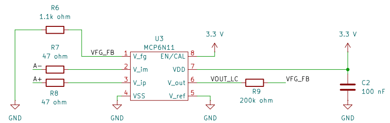
Functional Amplifier for the Load Cell
