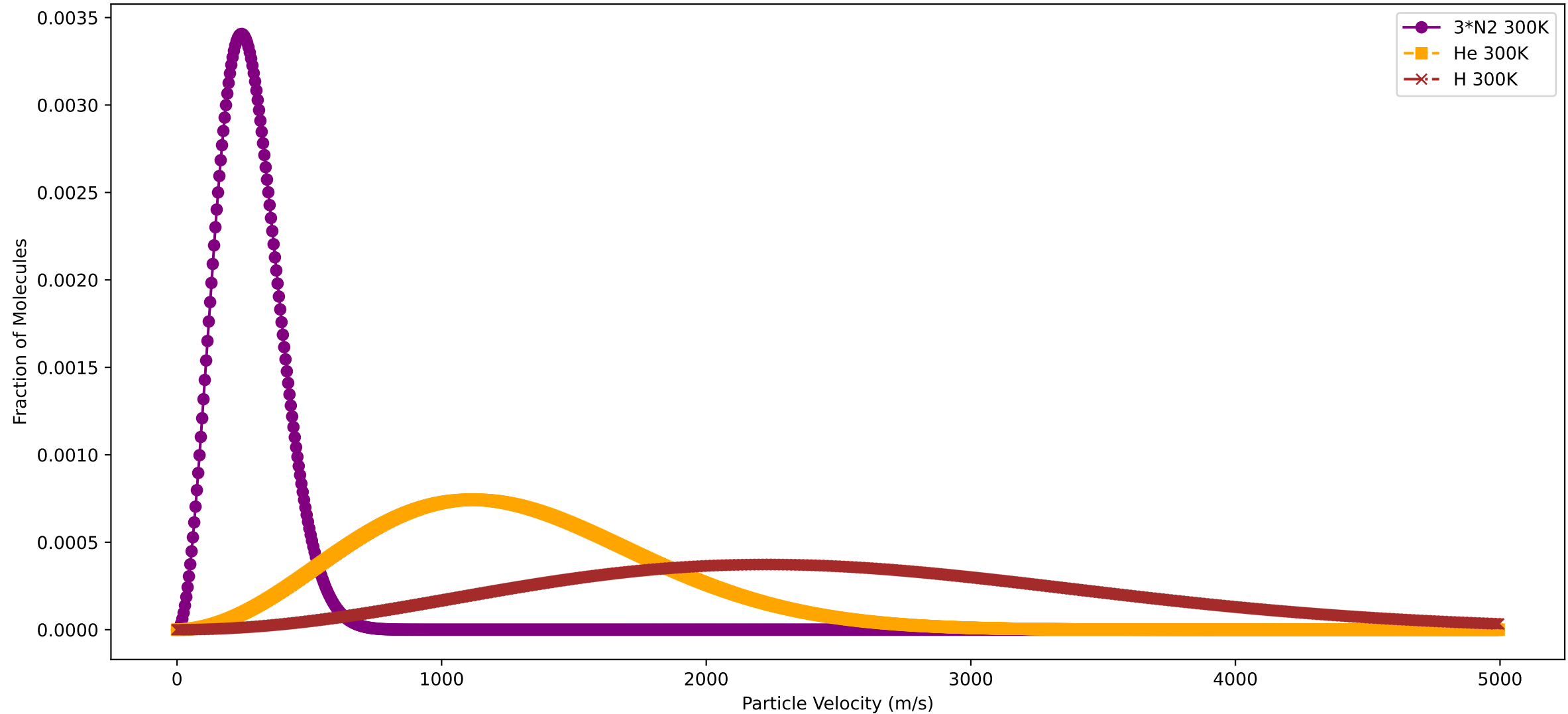
Maxwell Boltzmann Distribution for Varying Atomic Species at 300 K
