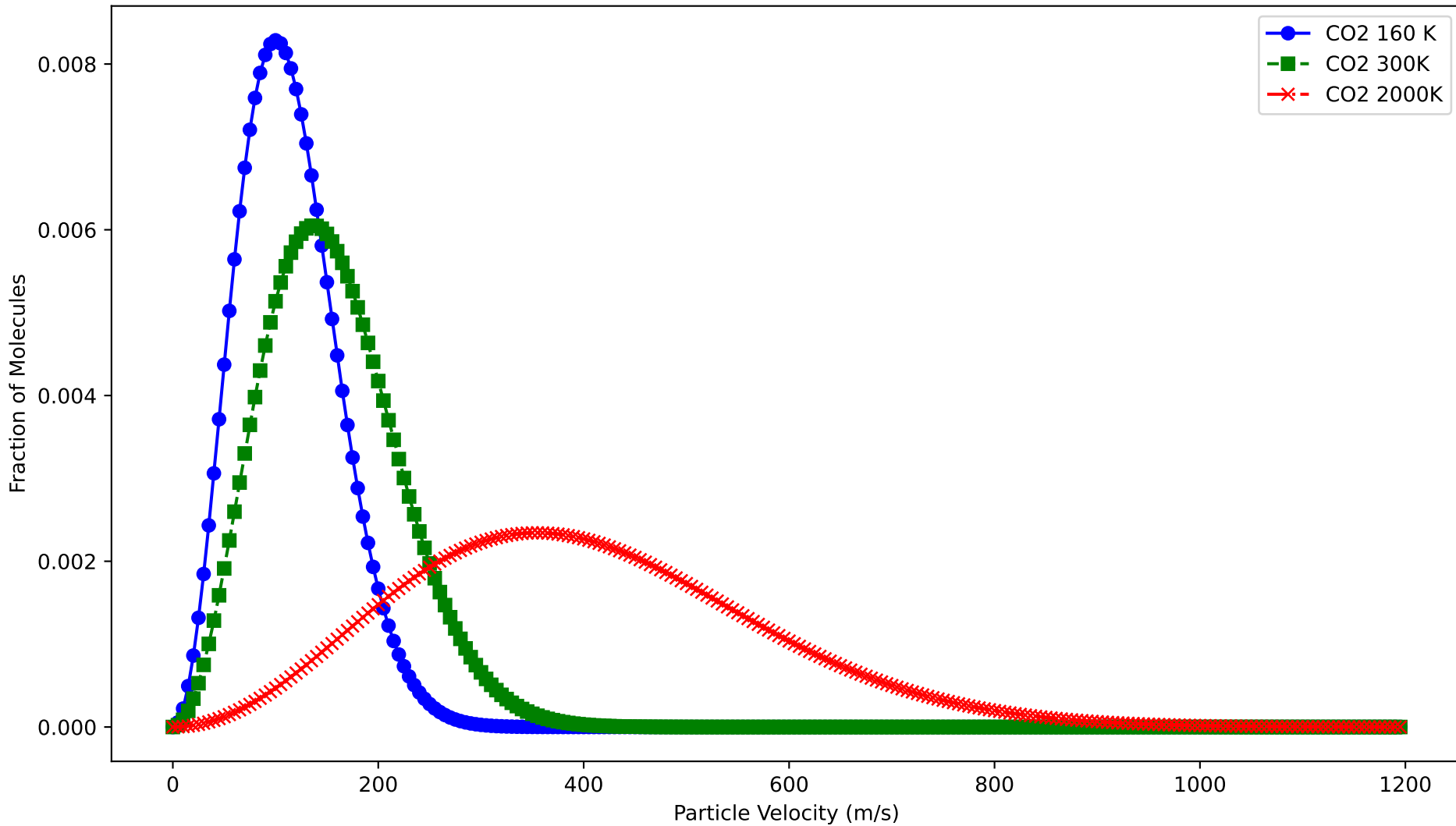
Maxwell Boltzmann Distribution for CO 2 at varying temperatures
