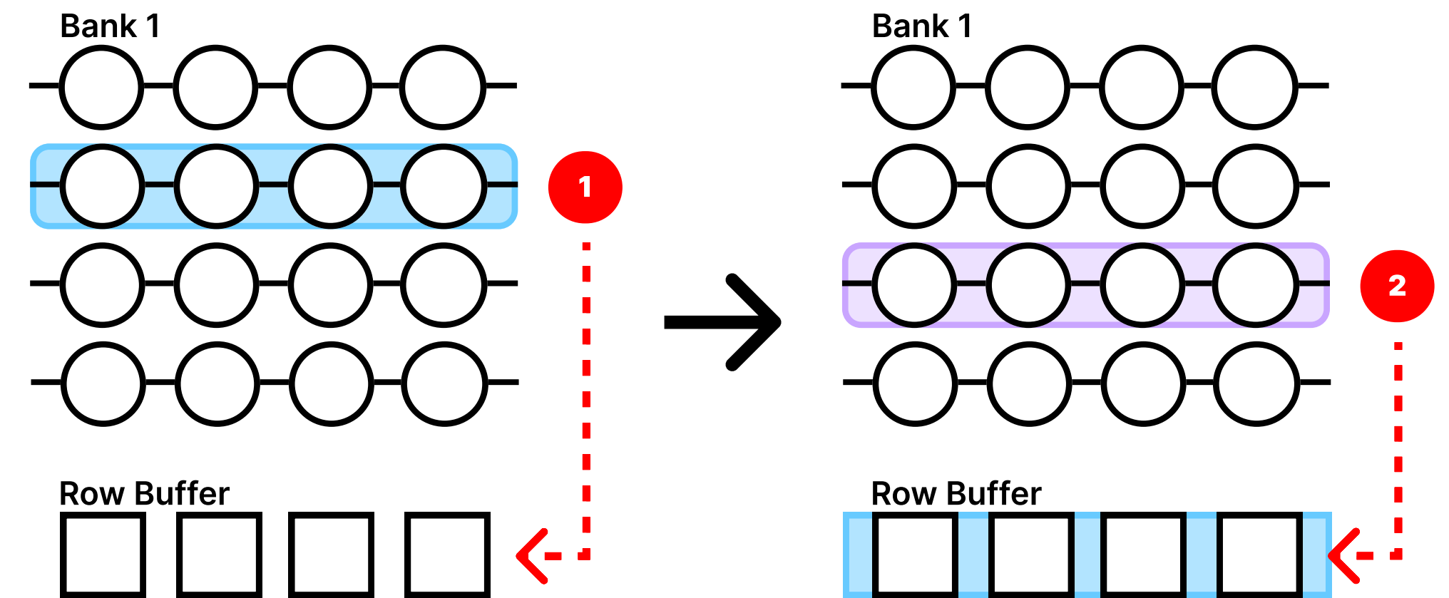
(c) Row Conflict
