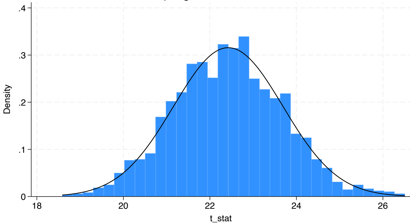
sampling distribution of t_stat
