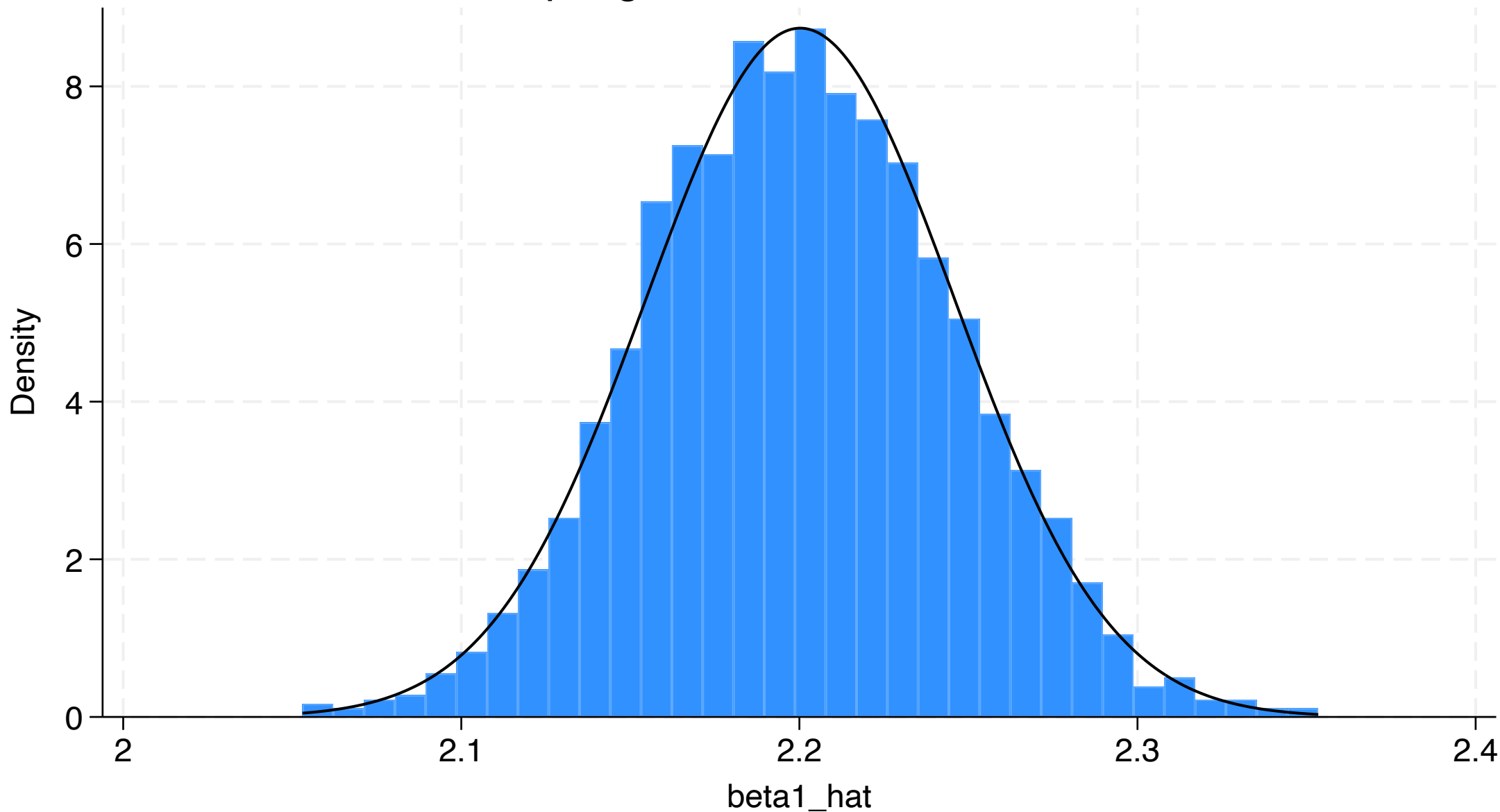
sampling distribution of beta1_hat
