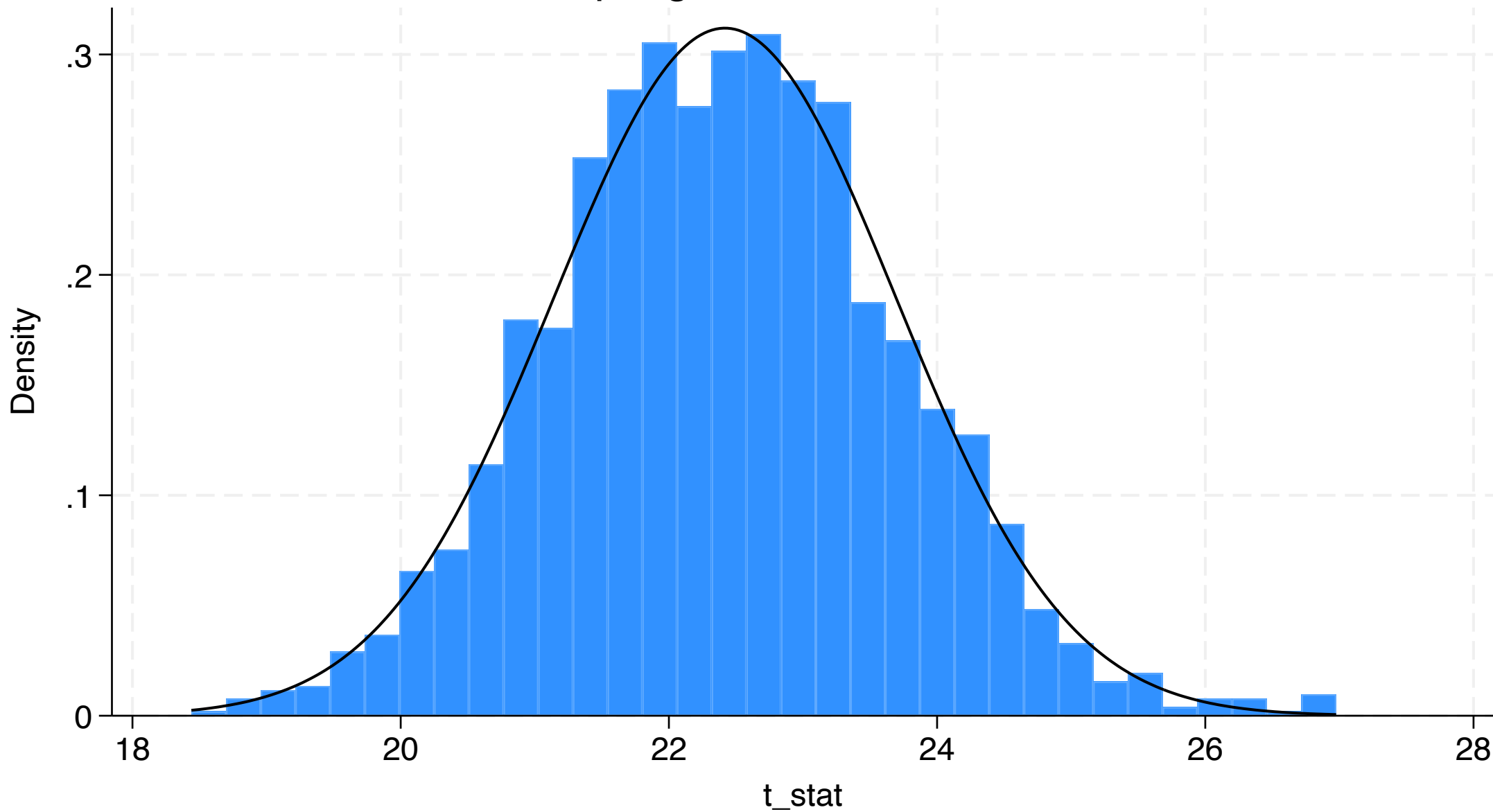
sampling distribution of t_{\text{stat}}
