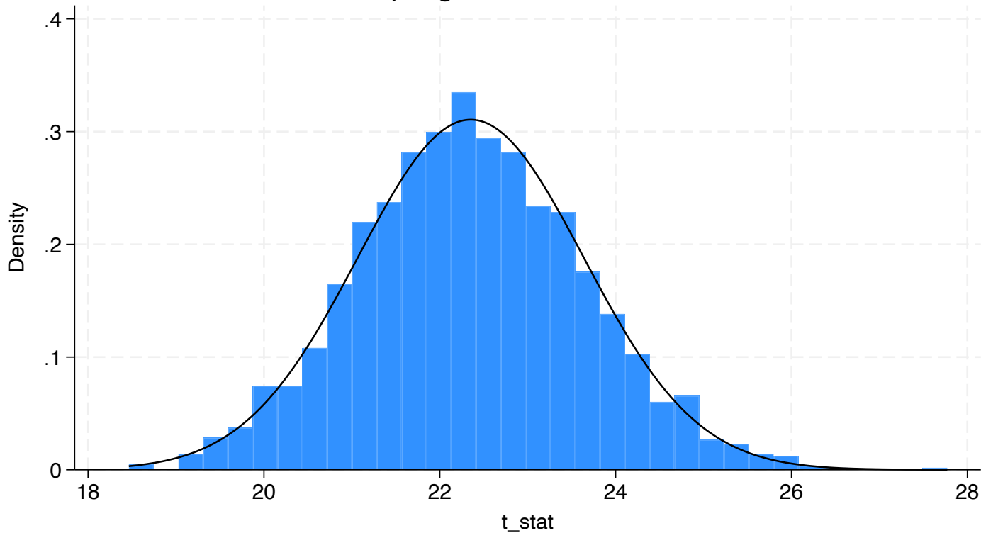
sampling distribution of t_{\text{stat}}
