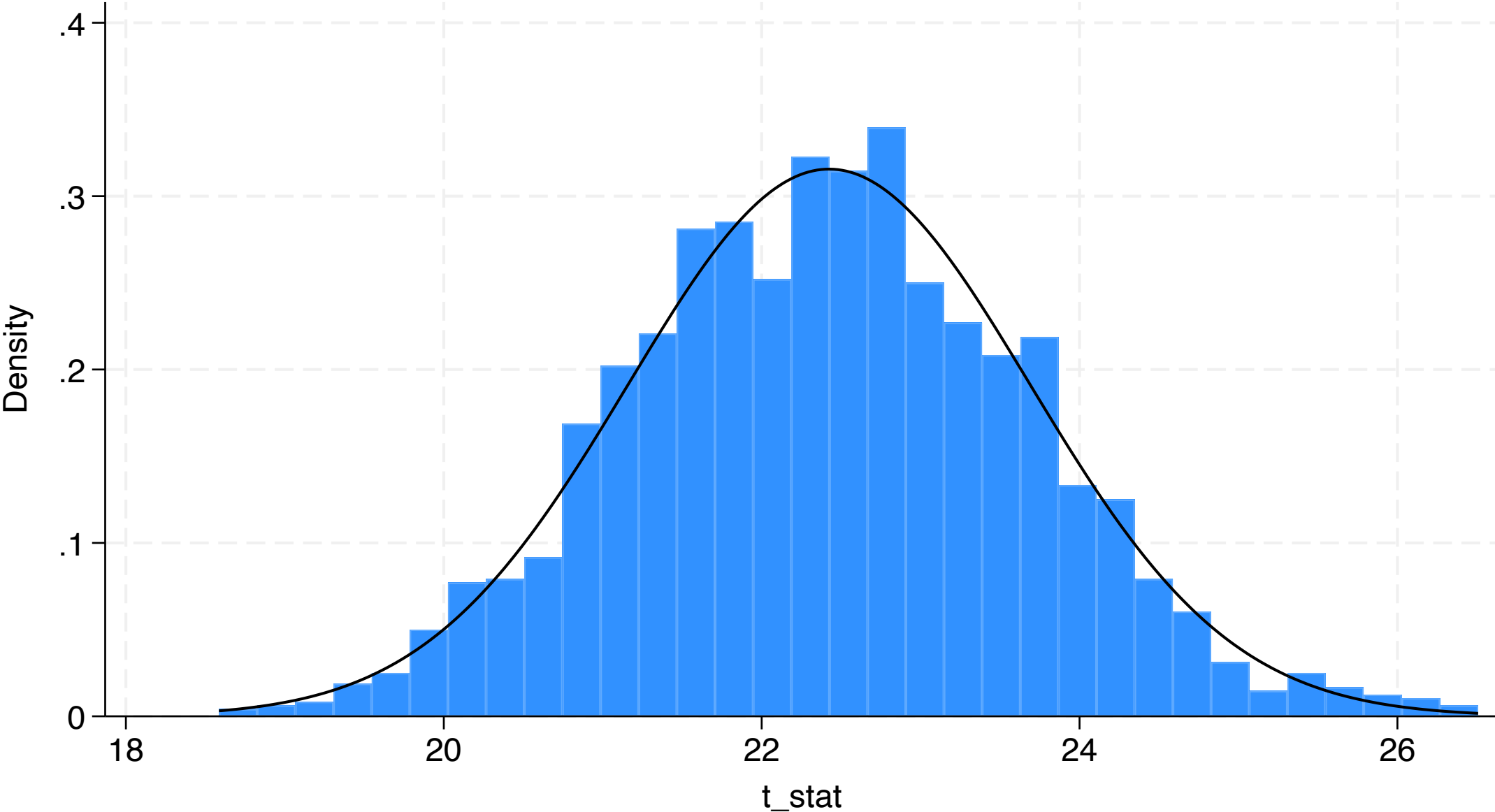
sampling distribution of t_stat
