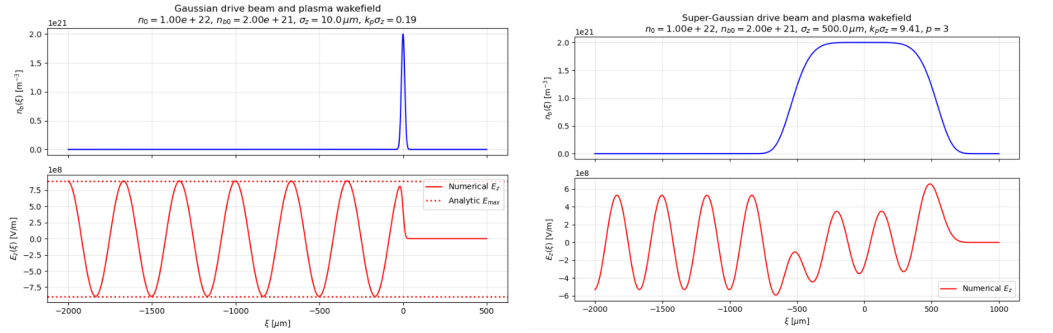
Figure 2: The electric fields E(\xi) with respect to a Gaussian and super-Gaussian drive beam.
