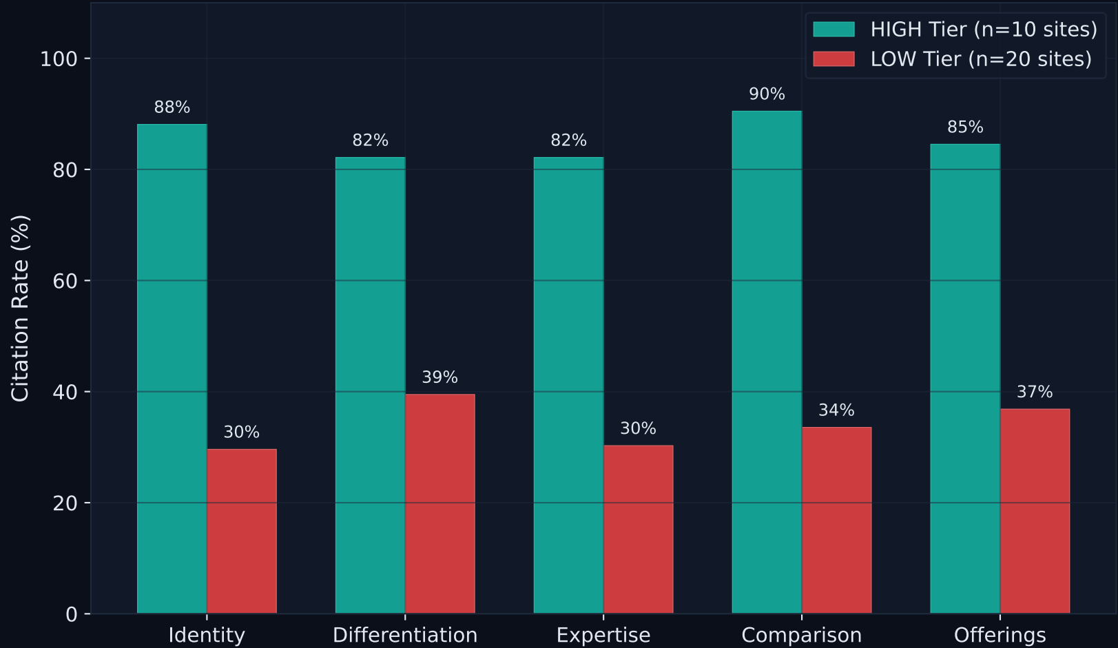
Citation Rate by Question Category and Site Tier
