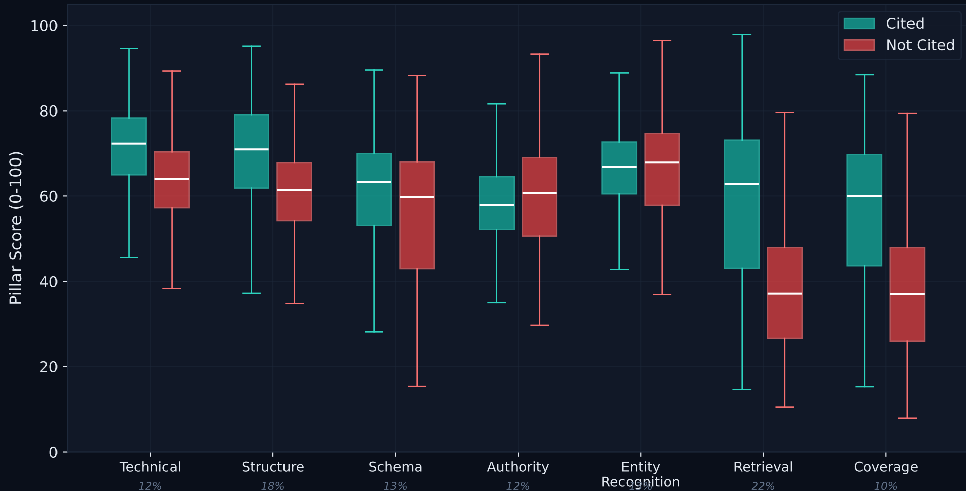
Pillar Score Distributions: Cited vs Uncited Sites
