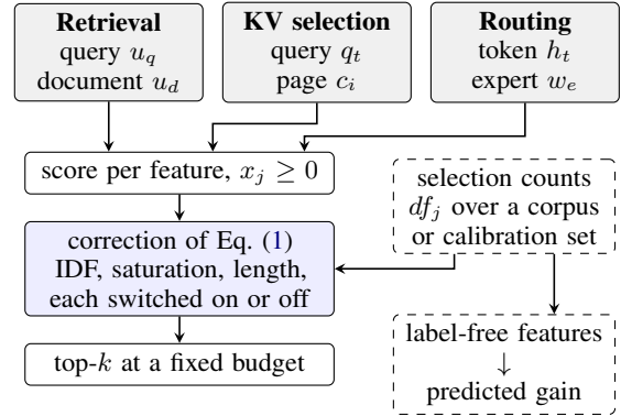
Figure 1: The computation shared by the three settings. Each scores an input against learned non-negative features and keeps the top k . The BM25 correction sits between the two steps. The selection counts it needs are also the input to the predictors of its gain.
