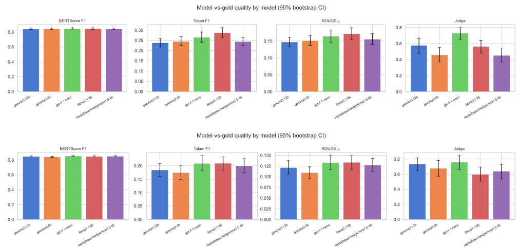
Figure 2. Model-vs-gold quality by model, with 95% bootstrap confidence intervals. BERTScore F1, Token F1, ROUGE-L, and LLM-judge score per model. (A) MedQuAD (top); (B) MedicationQA (bottom). BERTScore is tightly clustered across models; the closed reference GPT-4.1-nano leads on the judge score but remains within the open models' range on the other metrics.
