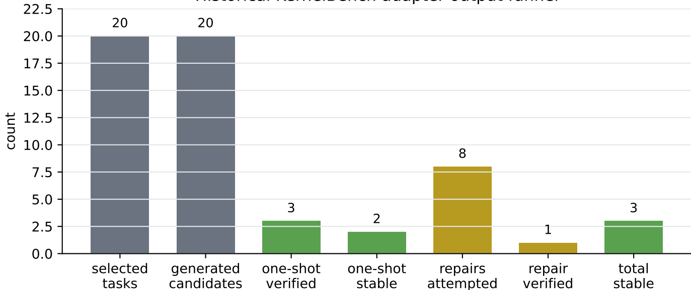
Historical KernelBench adapter output funnel
