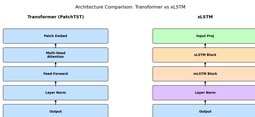
איור 3.1: Architecture Comparison: PatchTST vs xLSTM (Python-generated)
