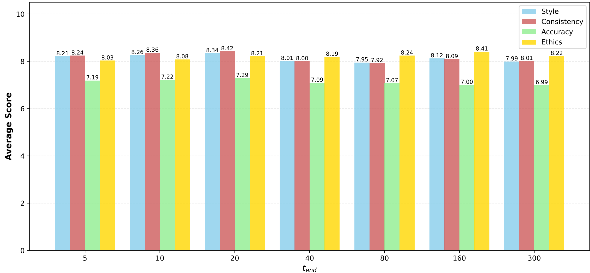
Evaluation Metrics vs t_{end}
