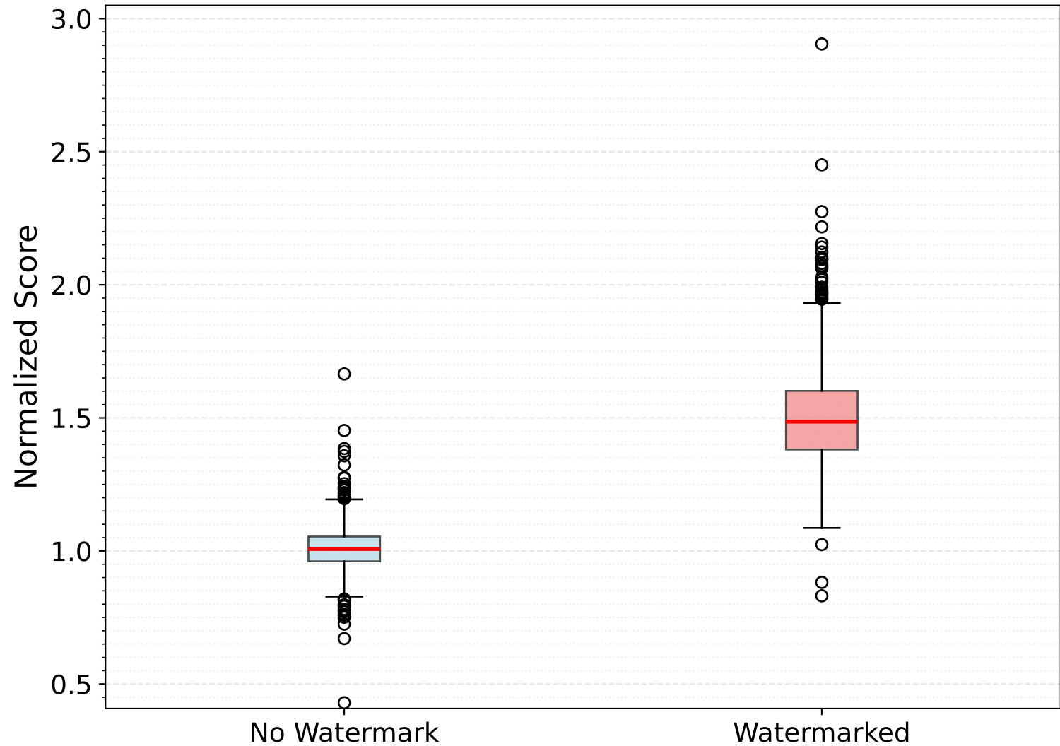
Watermark Detection Scores for 1000 Open-Ended Prompts
