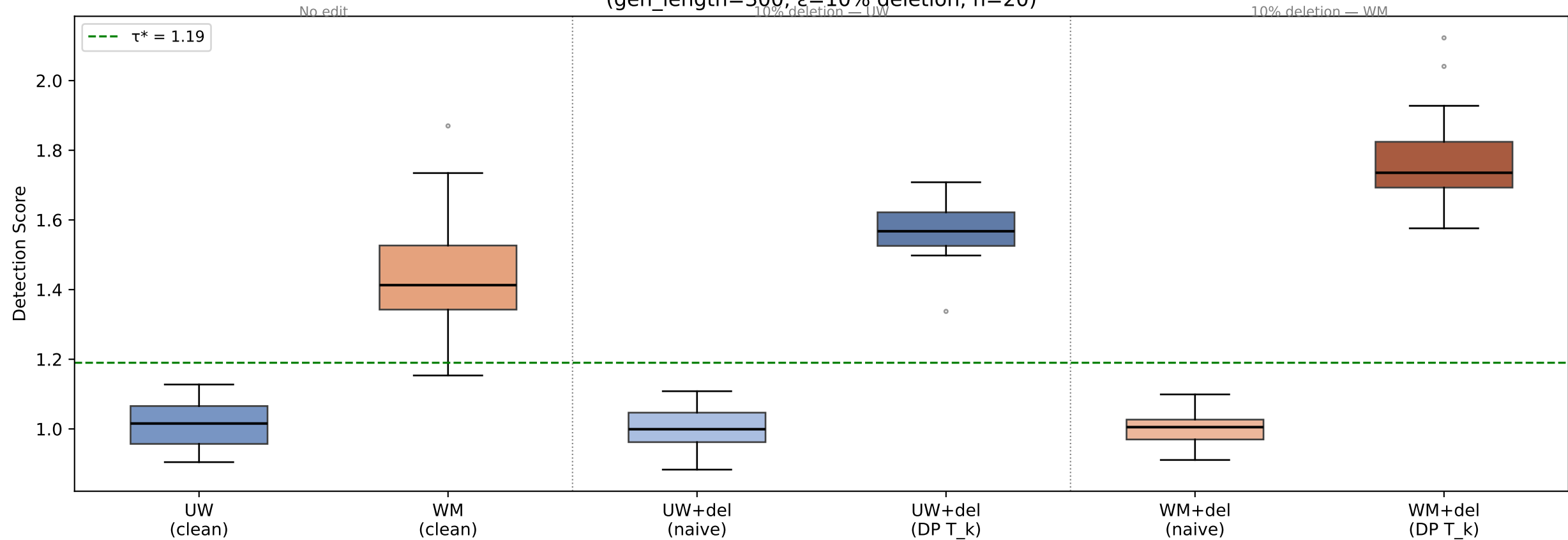
Gumbel-max Watermark Detection Scores: Naive vs DP Alignment (gen_length=300, \epsilon =10% deletion, n=20)
