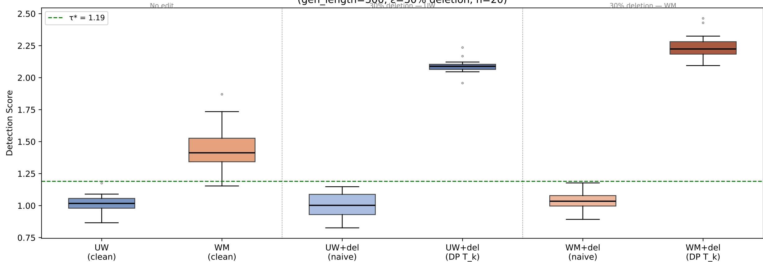
Gumbel-max Watermark Detection Scores: Naive vs DP Alignment (gen_length=300, \epsilon =30% deletion, n=20)
