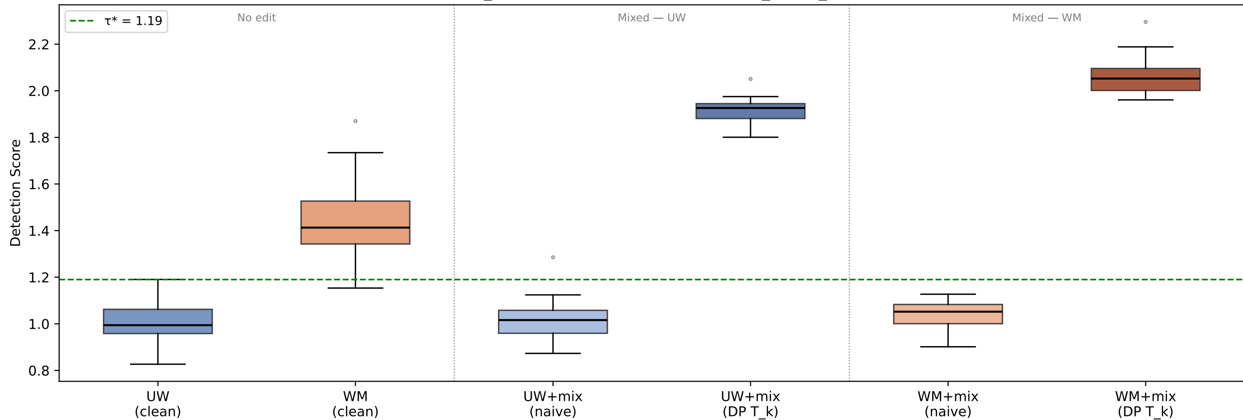
Gumbel-max Watermark Detection: Mixed Edits (sub=10%, del=10%, ins=10%) (gen_length=300, n=20, DP budget=n_del+n_ins)
