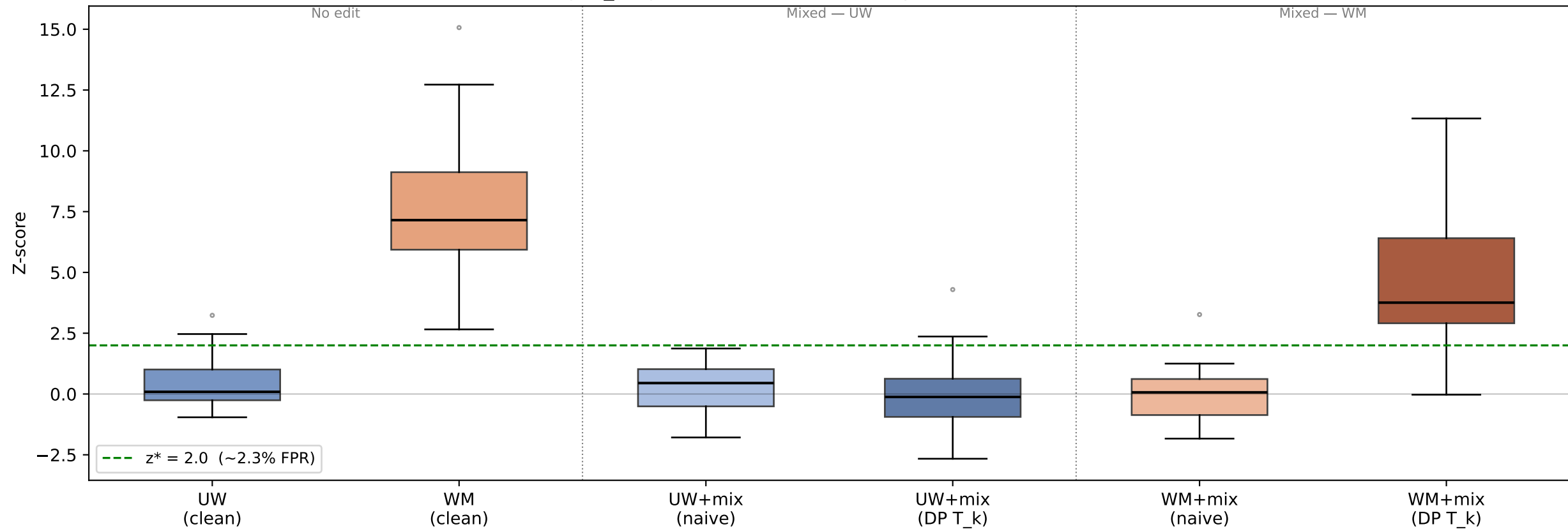
Gumbel-max Watermark Z-scores: Mixed Edits (sub=0%, del=10%, ins=0%) (gen_length=300, n=20, DP null: \mu=1.578 , \sigma=0.042 )
