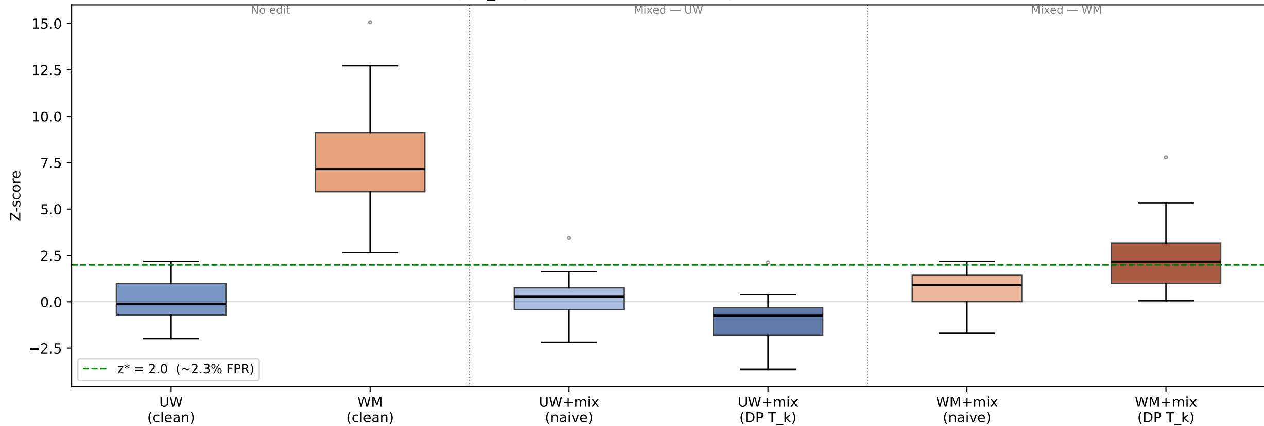
Gumbel-max Watermark Z-scores: Mixed Edits (sub=10%, del=10%, ins=10%) (gen_length=300, n=20, DP null: \mu=1.958 , \sigma=0.043 )
