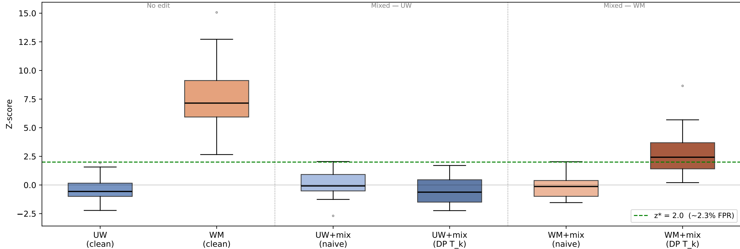
Gumbel-max Watermark Z-scores: Mixed Edits (sub=0%, del=30%, ins=0%) (gen_length=300, n=20, DP null: \mu=2.108 , \sigma=0.052 )
