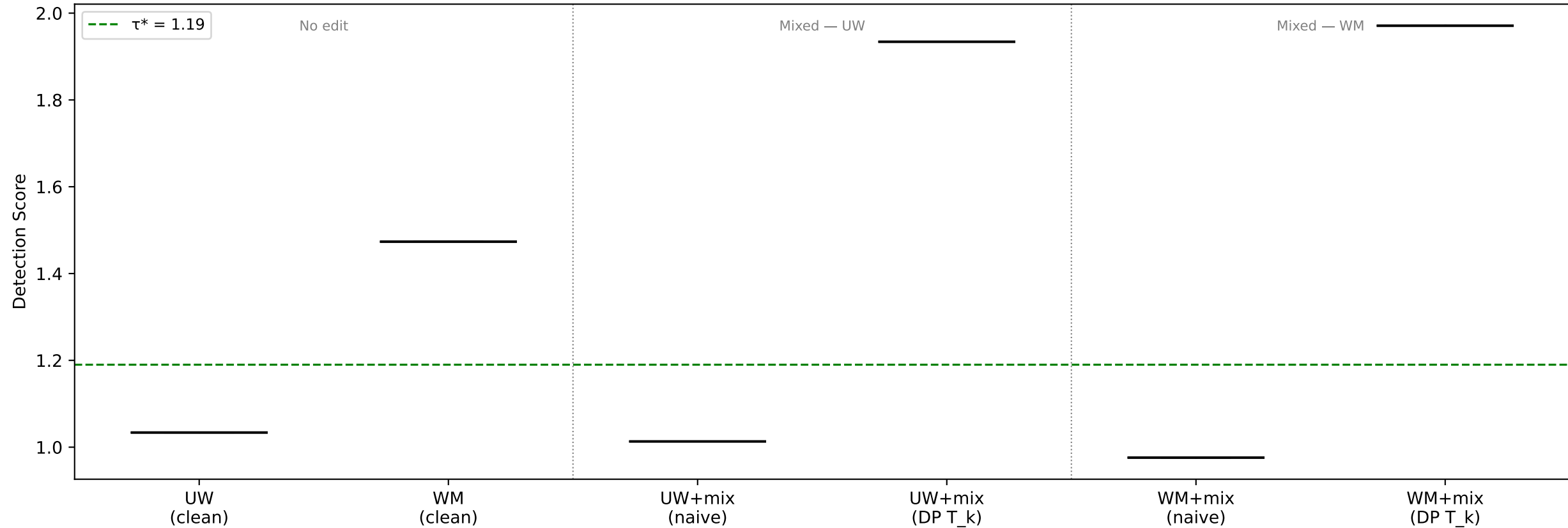
Gumbel-max Watermark Detection: Mixed Edits (sub=10%, del=10%, ins=10%) (gen_length=300, n=1, DP budget=n_del+n_ins)
