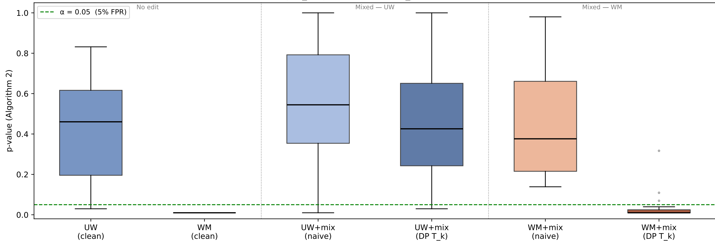
Gumbel-max Watermark p-values: Mixed Edits (sub=0%, del=0%, ins=10%) (gen_length=300, n=20, n_perms=100)
