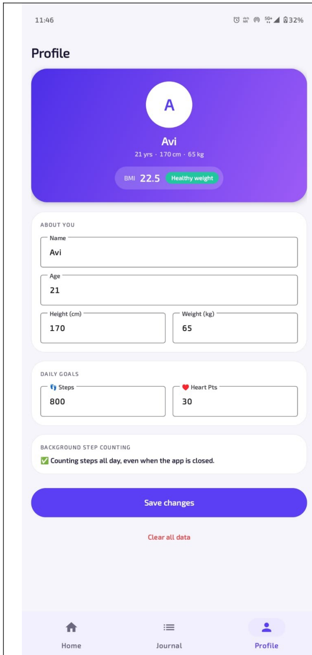
Profile Screen
