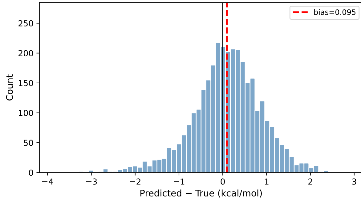
SaProt \Delta G residuals std=0.797
