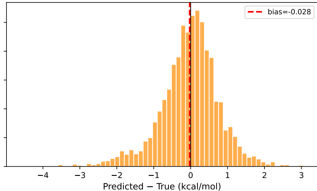
ESM3 \Delta G residuals std=0.801
