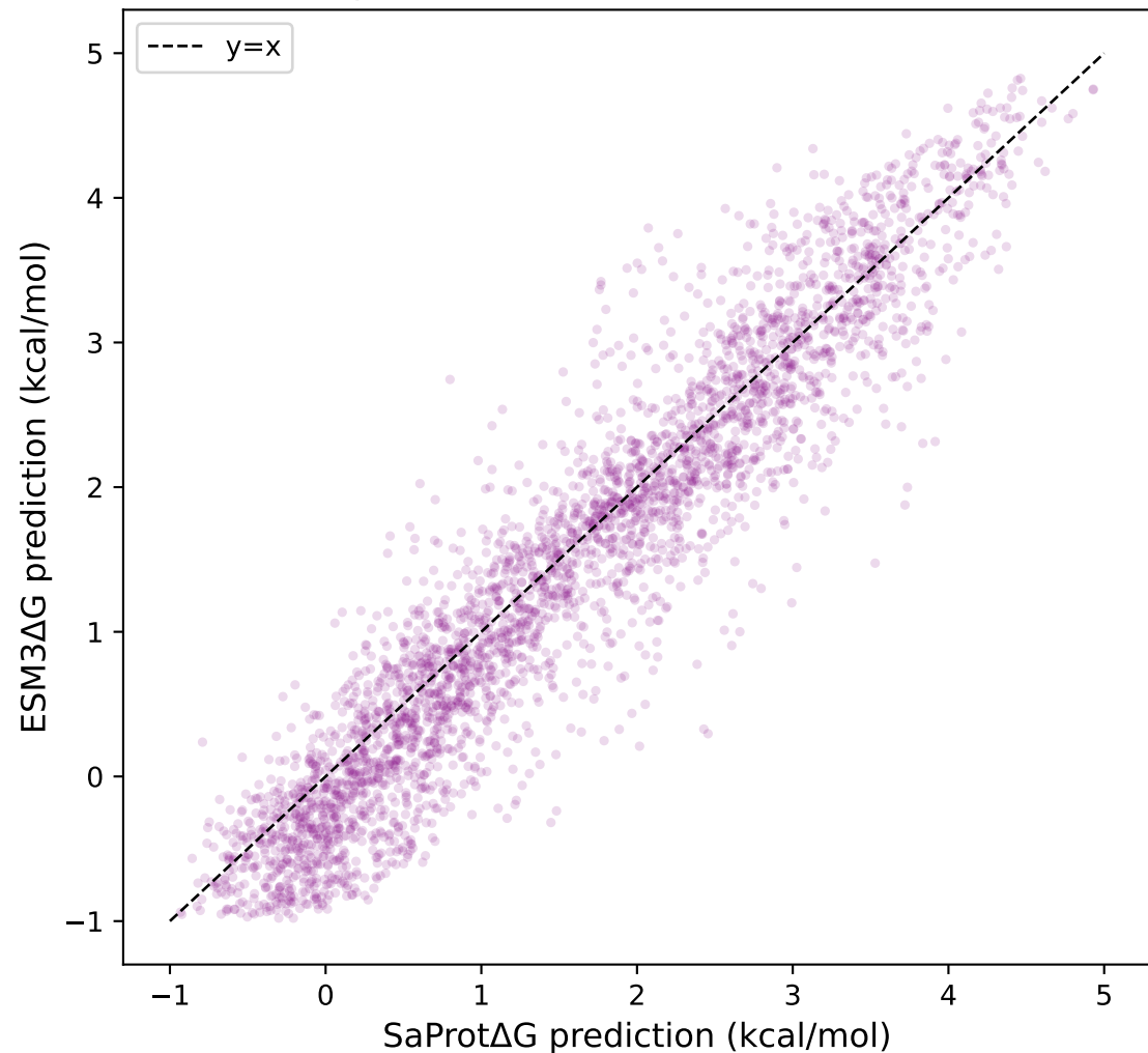
SaProt vs ESM3 predictions Spearman=0.9481 Pearson=0.9475
