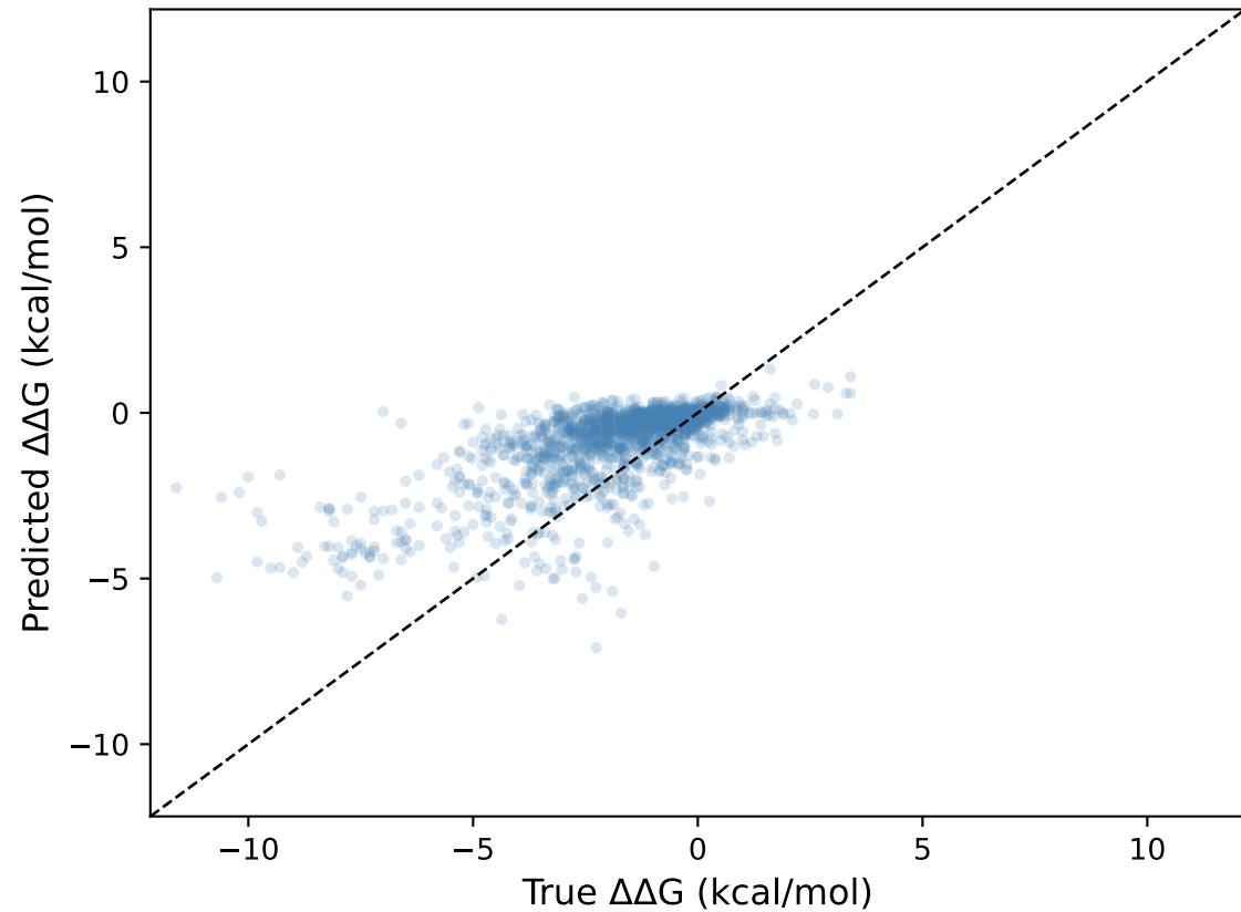
SaProt \Delta\Delta G \Delta\Delta G Spearman=0.6432 RMSE=1.6465
