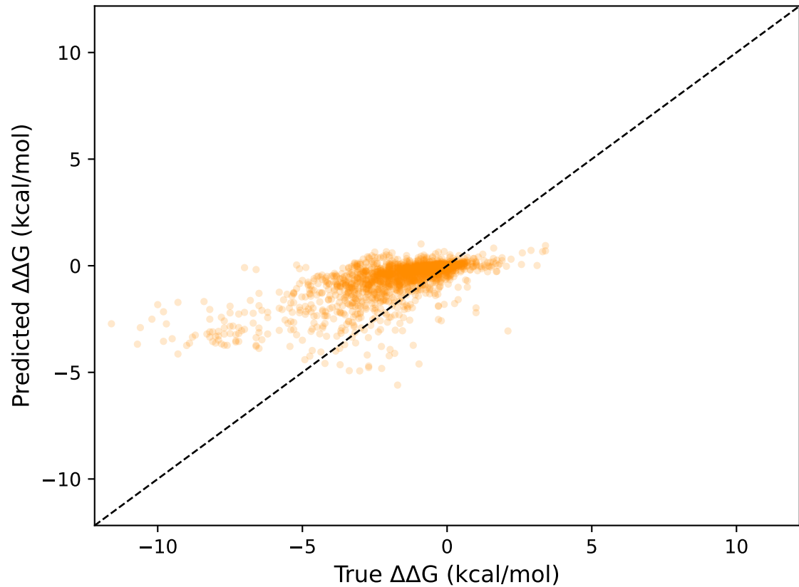
ESM3 \Delta\Delta G \Delta\Delta G Spearman=0.6620 RMSE=1.7740
