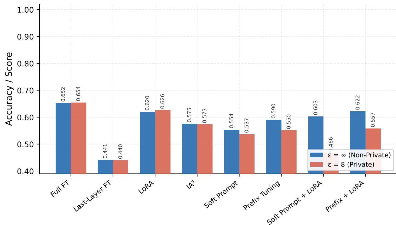
MNLI
