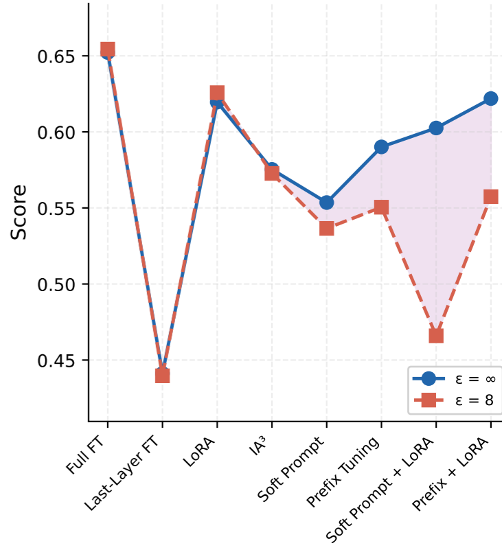
MNLI
