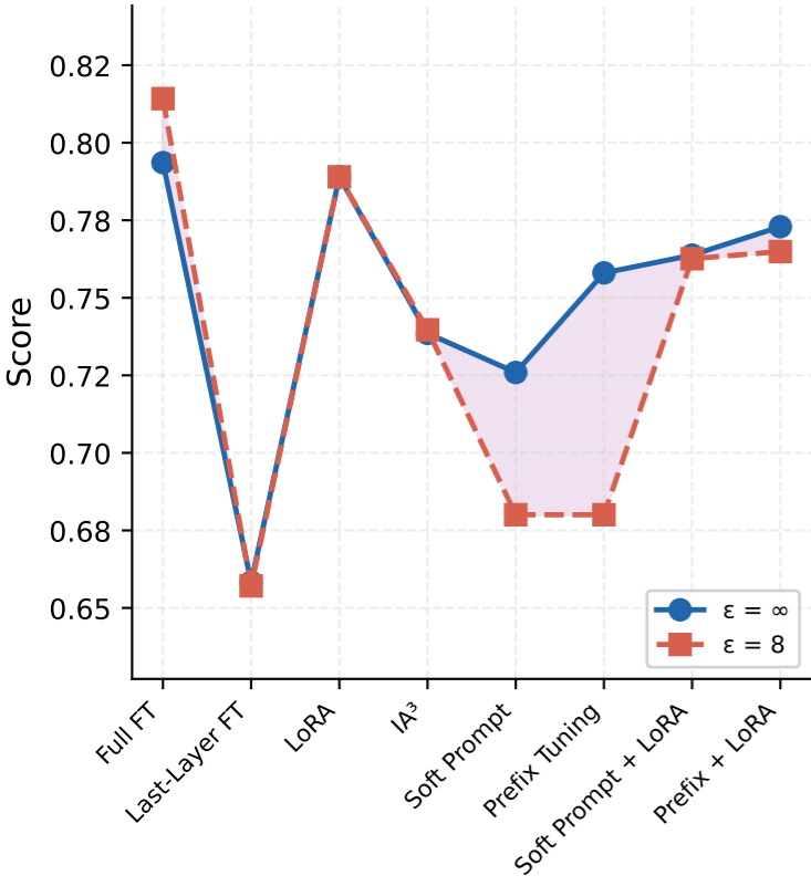
SST-2
