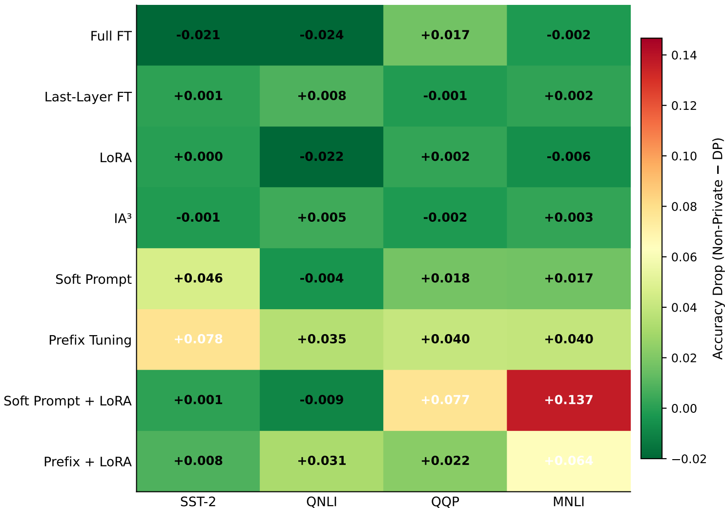
Privacy Cost: Accuracy Drop when Adding DP ( \epsilon = 8 )
