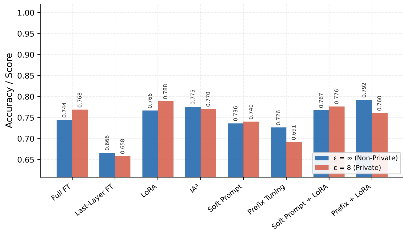
MNLI
