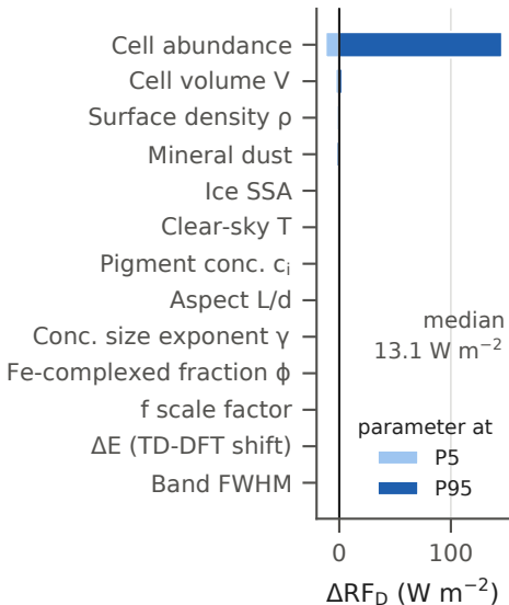
a One-at-a-time
