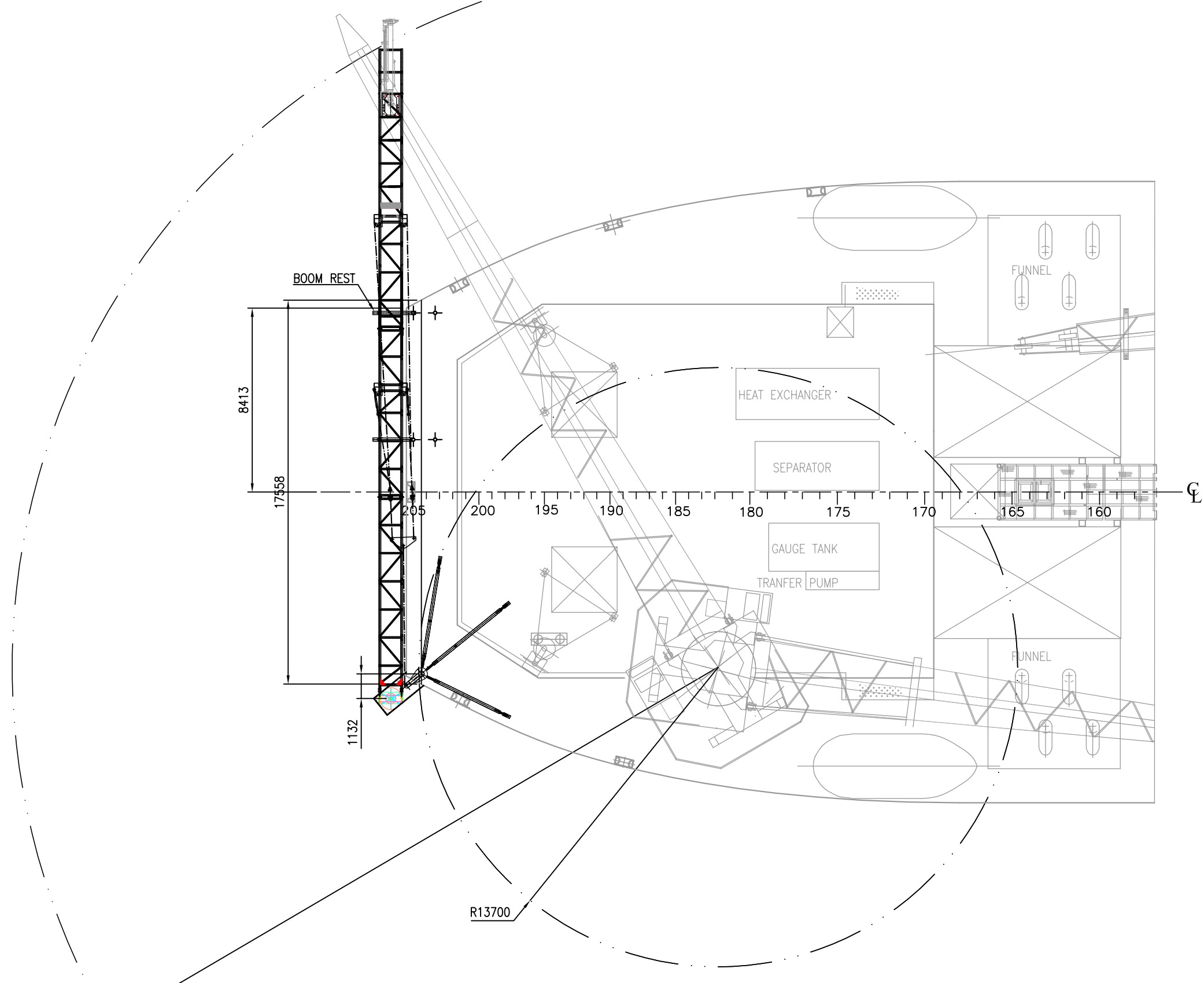
PLAN VIEW BURNER BOOM AT STACKING POSITION (Scale 1:200)
