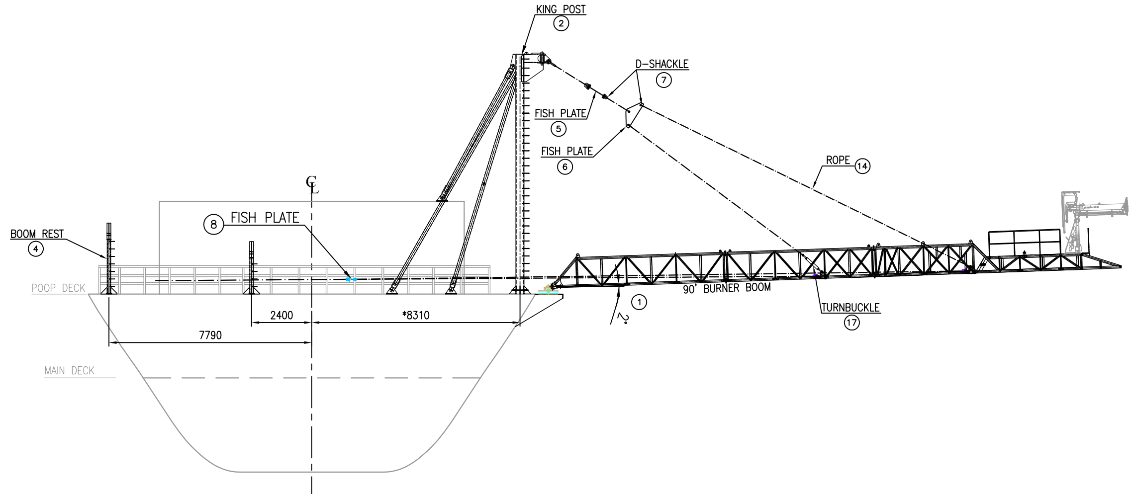
TRANSOM SECTION BURNER BOOM AT OPERATING POSITION (Scale 1:150)
