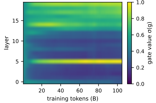
Figure 6: Gate values over training, SAN 105B run (layers \times time). Early layers self-attenuate and late layers sharpen under Muon.
