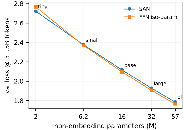
Figure 2: Iso-token scaling (31.5B tokens per size). The SAN wins at the smallest size; from 16M non-embedding parameters upward the gap is flat at \approx 0.02 nats.
