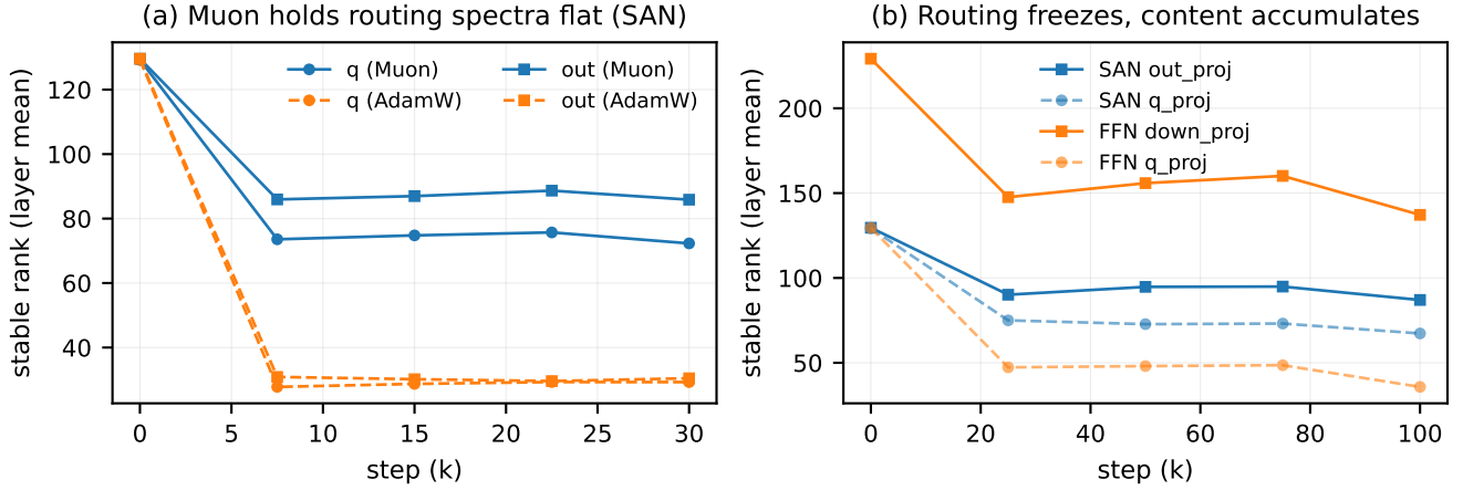
Figure 5: Stable rank ( \|W\|_F^2/\|W\|_2^2 , layer mean) of weight matrices over training. (a) Muon holds Q and output-projection spectra 2\text{--}3\times flatter than AdamW in the SAN. (b) Routing matrices (Q) crystallize by a quarter of training in every model; write-path matrices (SAN W_o , FFN down-projection) accumulate rank through the stable phase, contracting only in the learning-rate decay tail.
