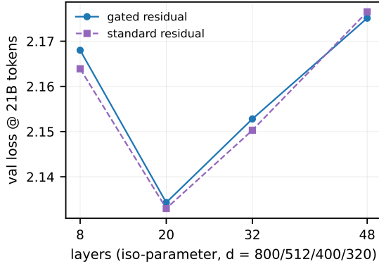
Figure 8: Iso-parameter depth ladder for the SAN arm, gated vs. standard residuals: U-shaped in depth with a 20-layer optimum; gates neutral at every depth; 48 layers train without incident.
