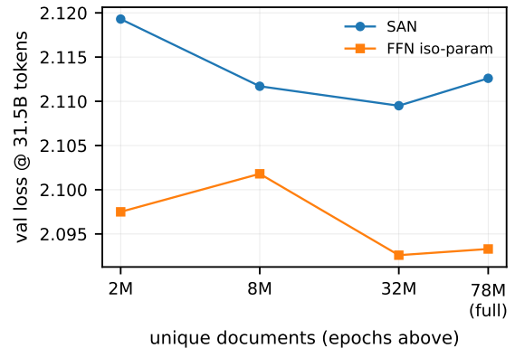
Figure 3: Unique-document constraints at a fixed 31.5B-token budget. Both arms are nearly repetition-insensitive, with no architecture interaction.
