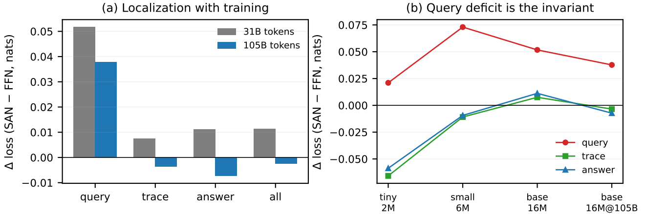
Figure 4: (a) Region-level gap at 31B vs. 105B tokens: with training the deficit localizes entirely to low-context query prediction. (b) Across matched size pairs, the query deficit is the only invariantly FFN-favored quantity.
