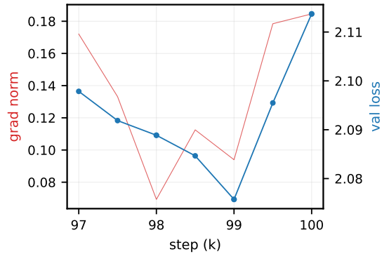
Figure 7: The FFN iso-param seed-43 terminal instability. The run tracked its sibling seed to within 0.002 nats through step 99,000. Its final value is included, flagged, in all statistics.
