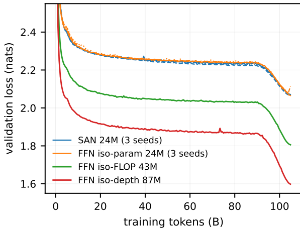
Figure 1: Validation loss over 105B tokens: three SAN seeds, three FFN iso-param seeds, and the iso-FLOP and iso-depth controls. The iso-param pair is visually indistinguishable through training.
