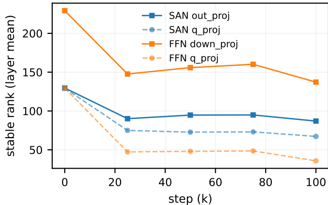
(b) Routing freezes, content accumulates
