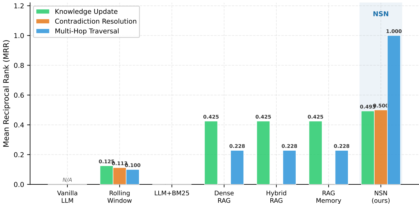
MRR Across Seven Systems and Three Benchmarks
