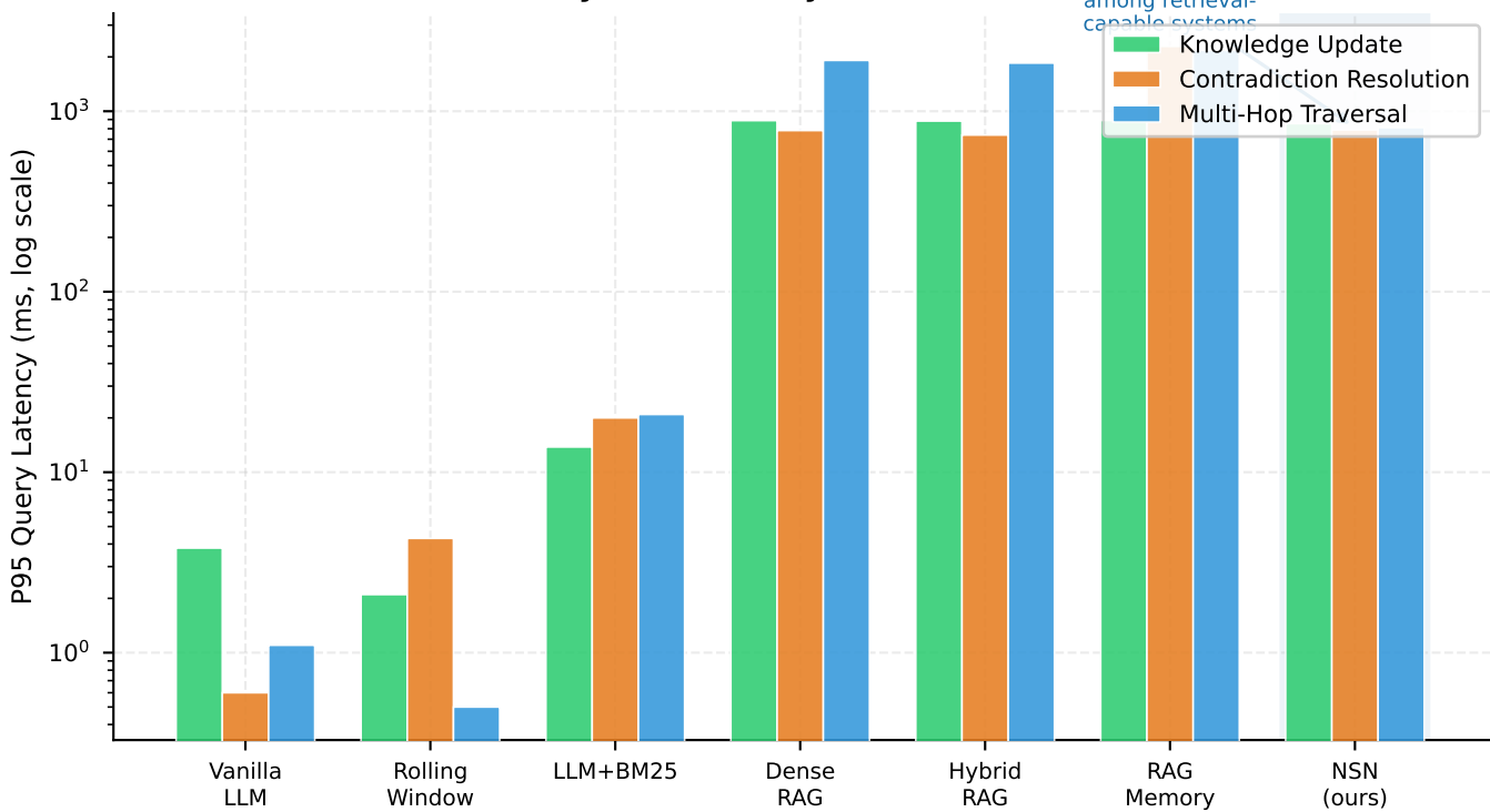
P95 Latency Across All Systems and Benchmarks
