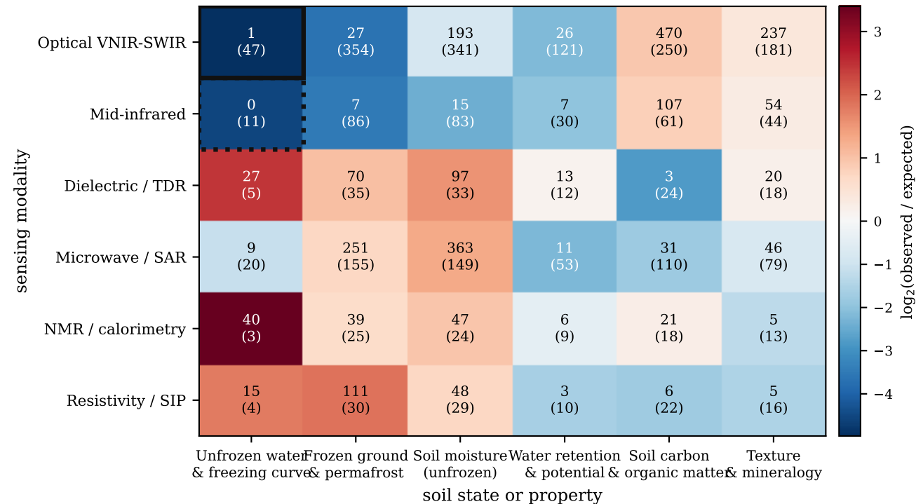
Co-occurrence of sensing modality and soil state in 9021 works cell shows observed count (expected under independence)
