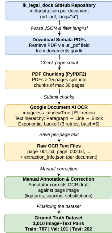
Fig. 1. Document processing pipeline for constructing the Sinhala government acts OCR dataset.
