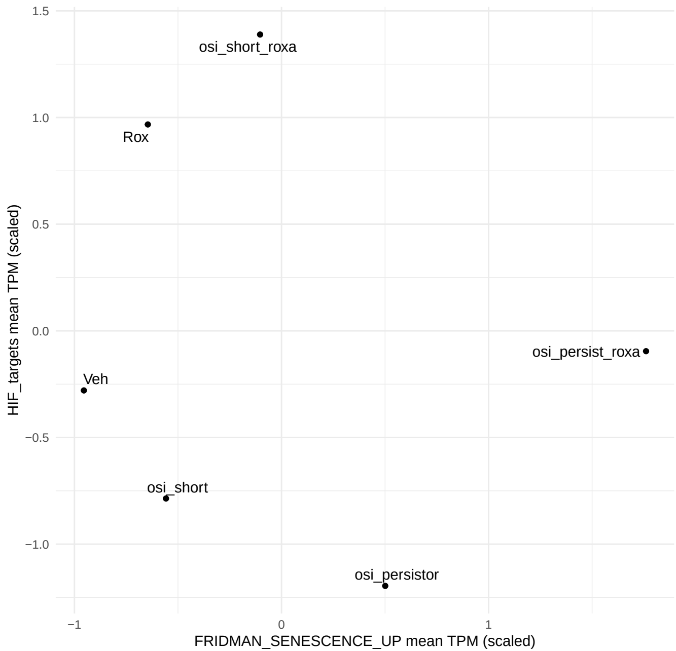
H1975: FRIDMAN_SENESCENCE_UP vs HIF_targets
