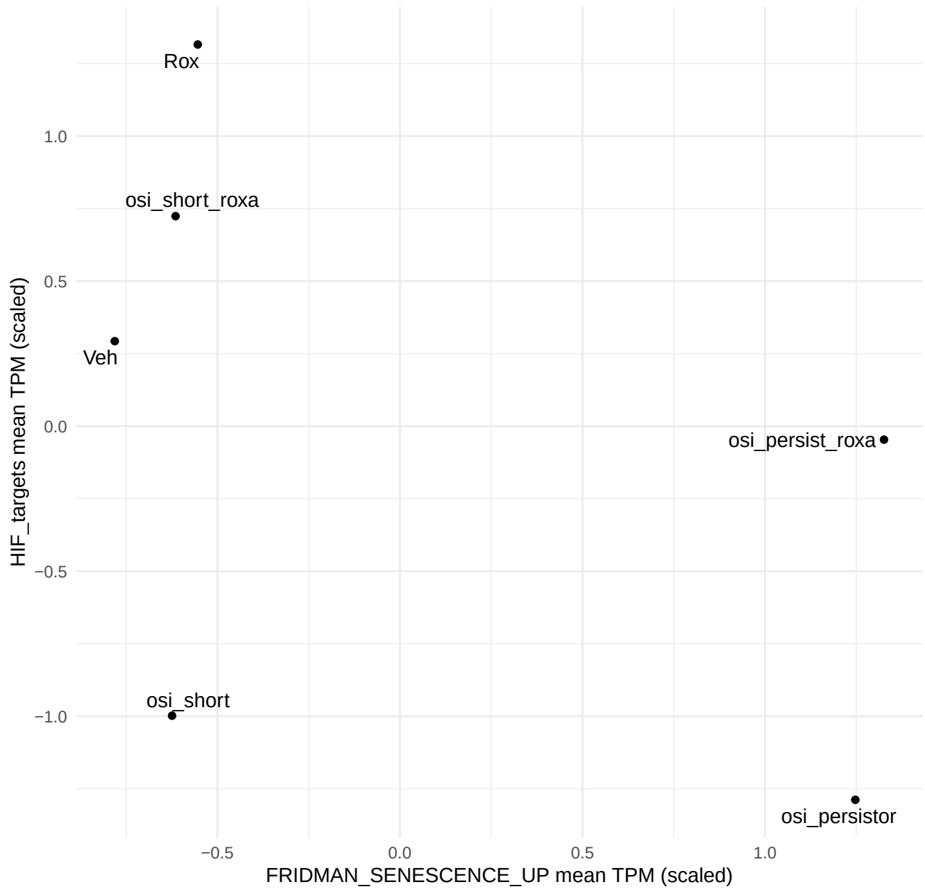
HCC827: FRIDMAN_SENESCENCE_UP vs HIF_targets
