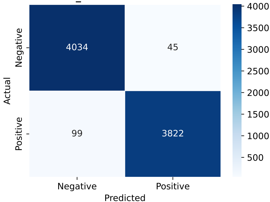
Custom_CNN - Confusion Matrix
