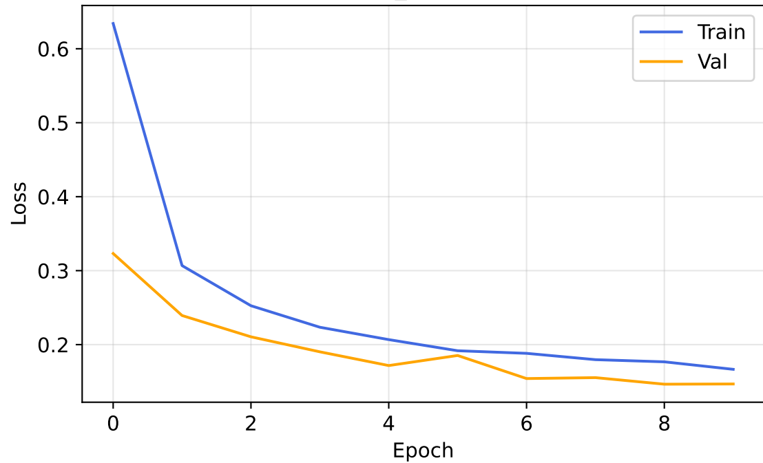
Custom_CNN - Loss
