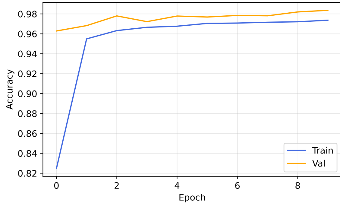
Custom_CNN - Accuracy
