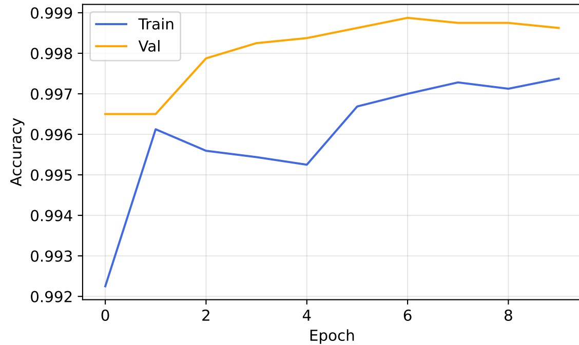
MobileNetV2 - Accuracy
