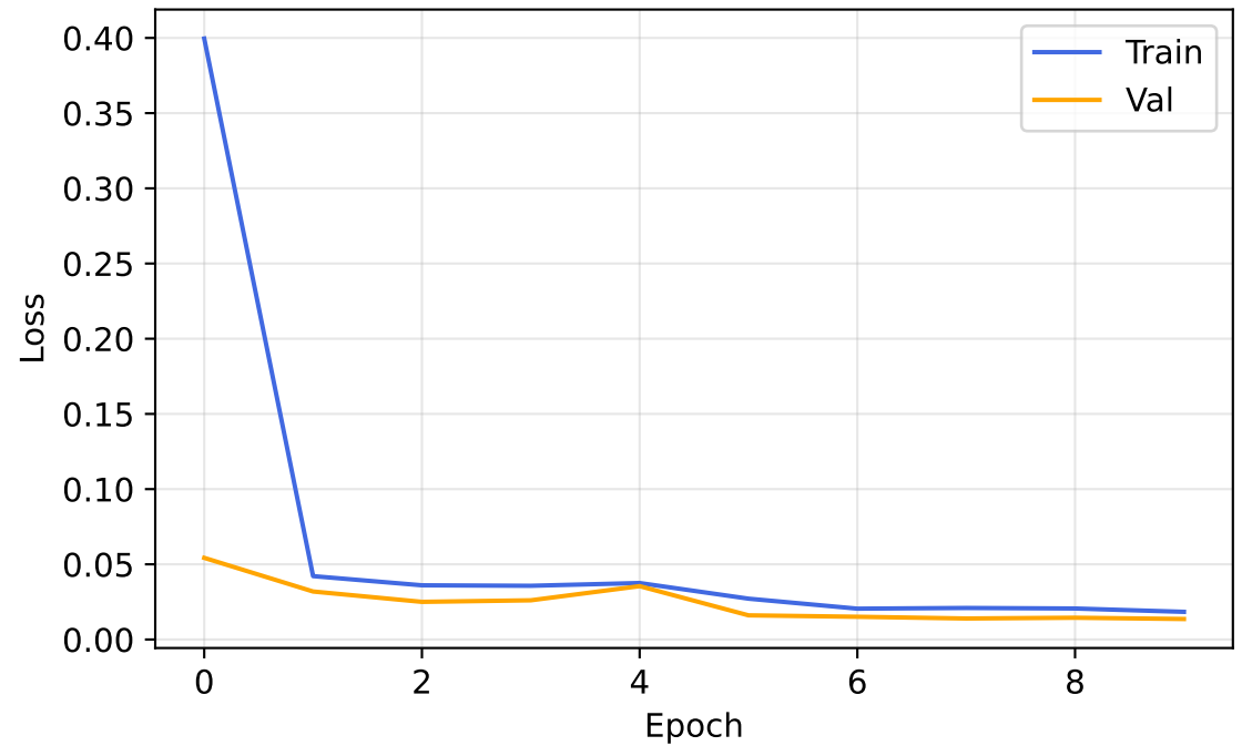
MobileNetV2 - Loss
