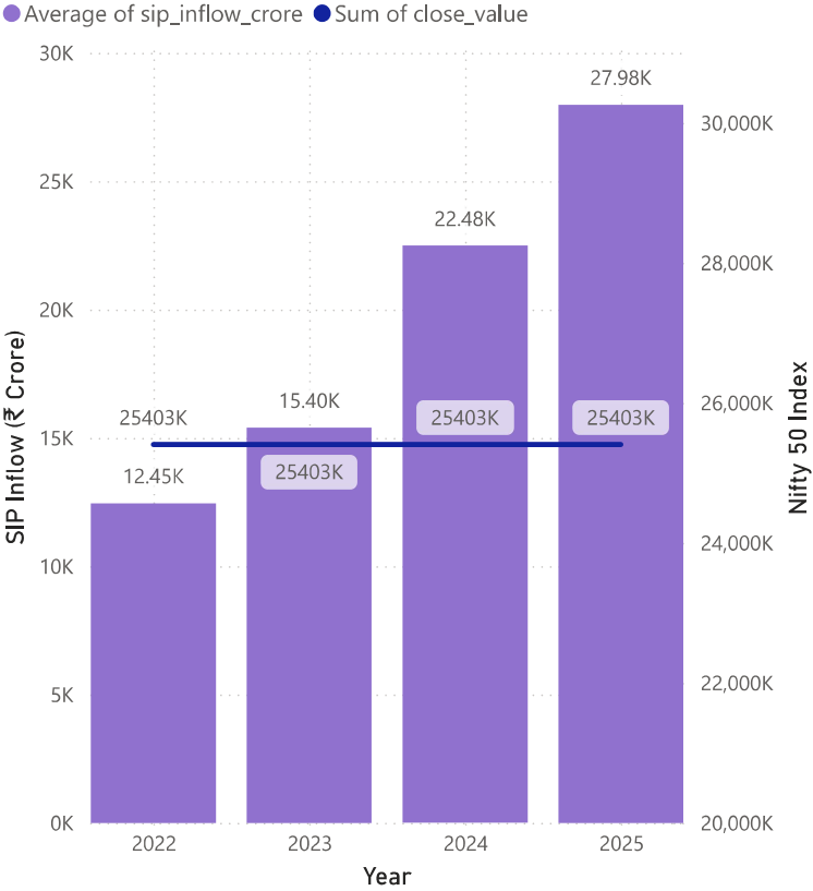
SIP Inflows vs Nifty 50 Trend (2022–2025)
